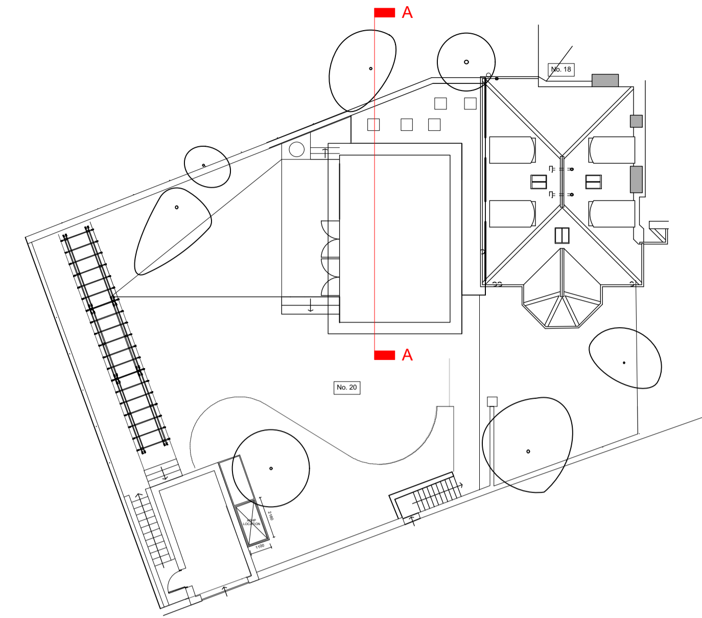
KEY PLAN 1:200
