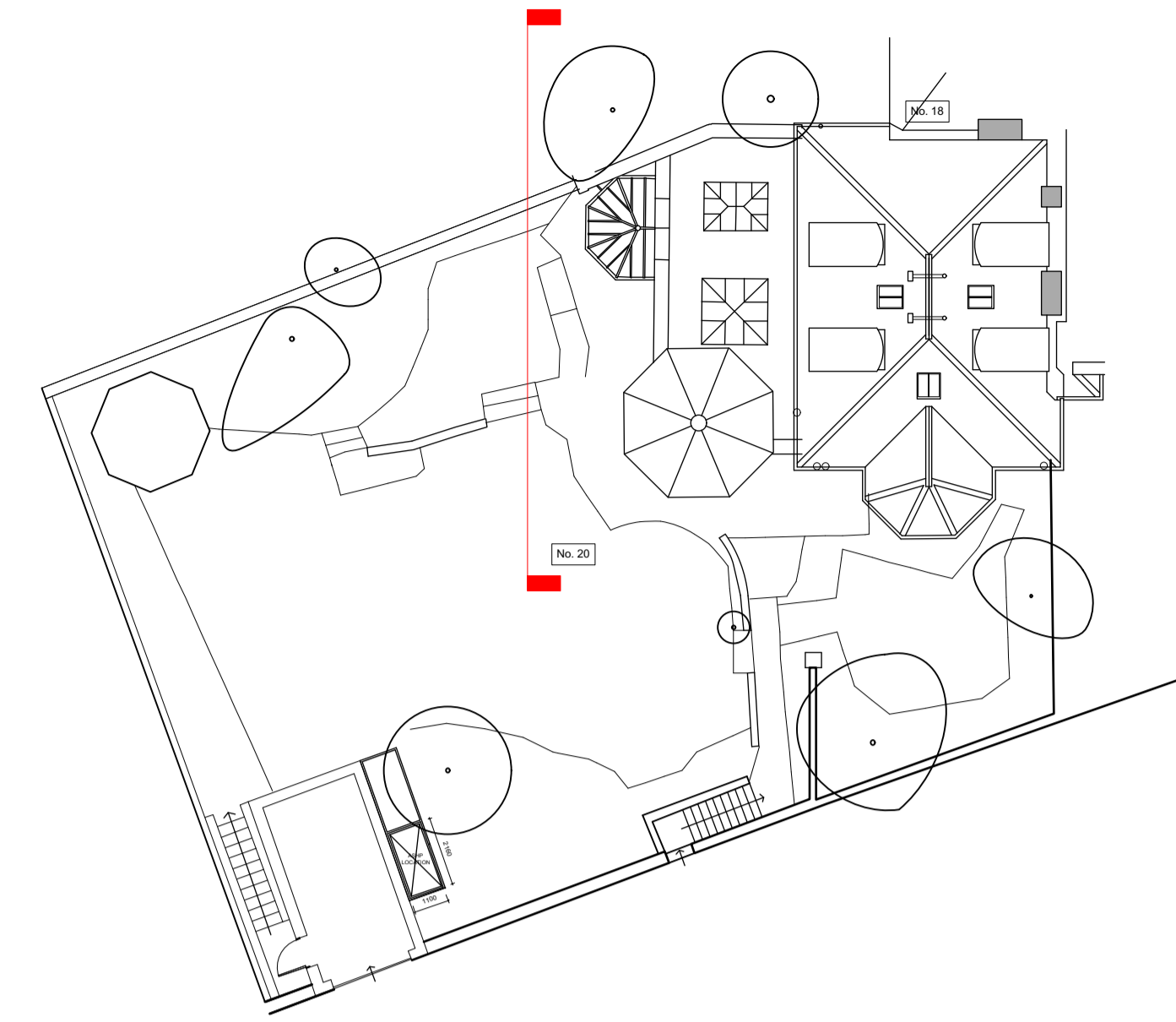
KEY PLAN 1:200
