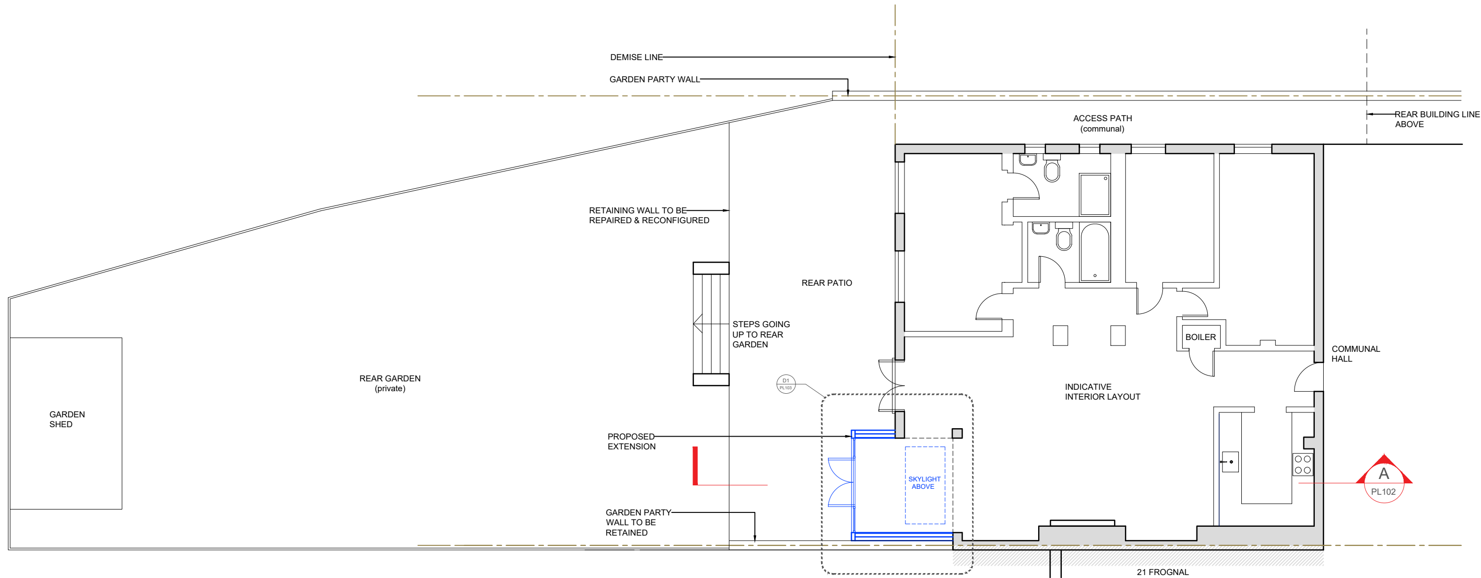
LOWER GROUND FLOOR PLAN AS PROPOSED
