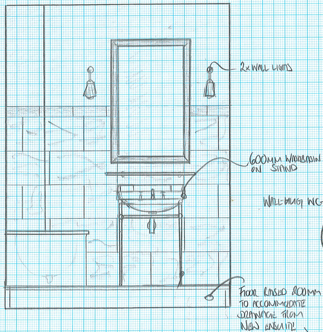
WEST ELEVATION
