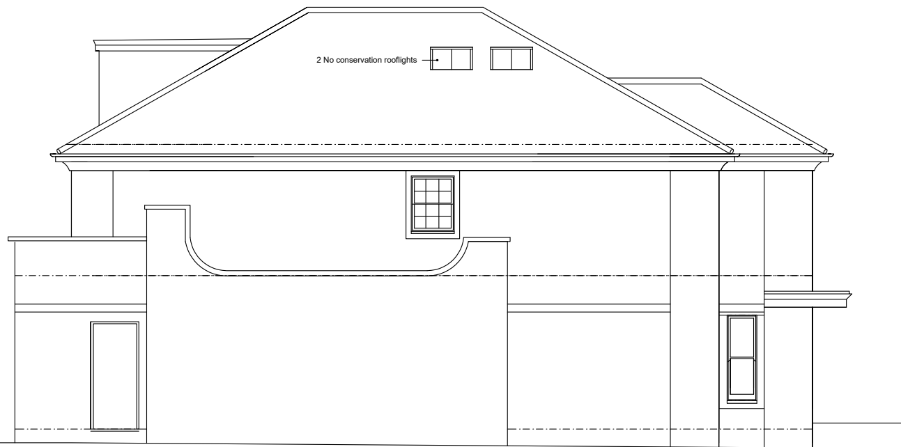
side elevation
