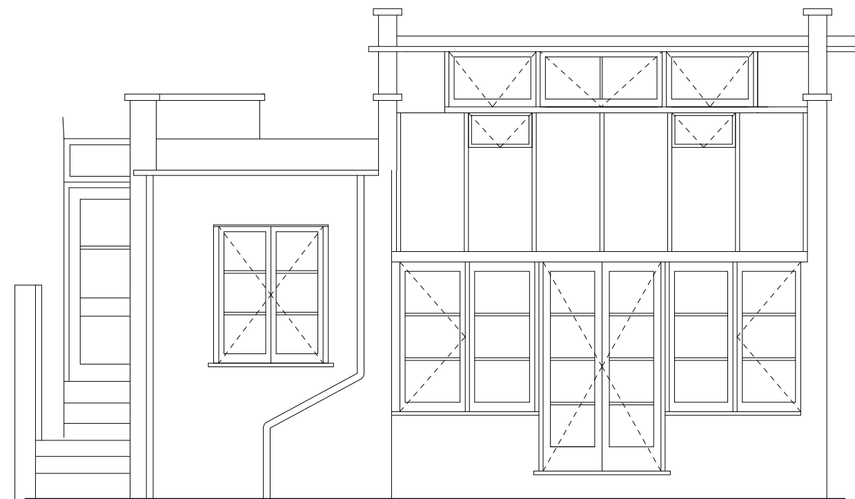
Existing Elevation
