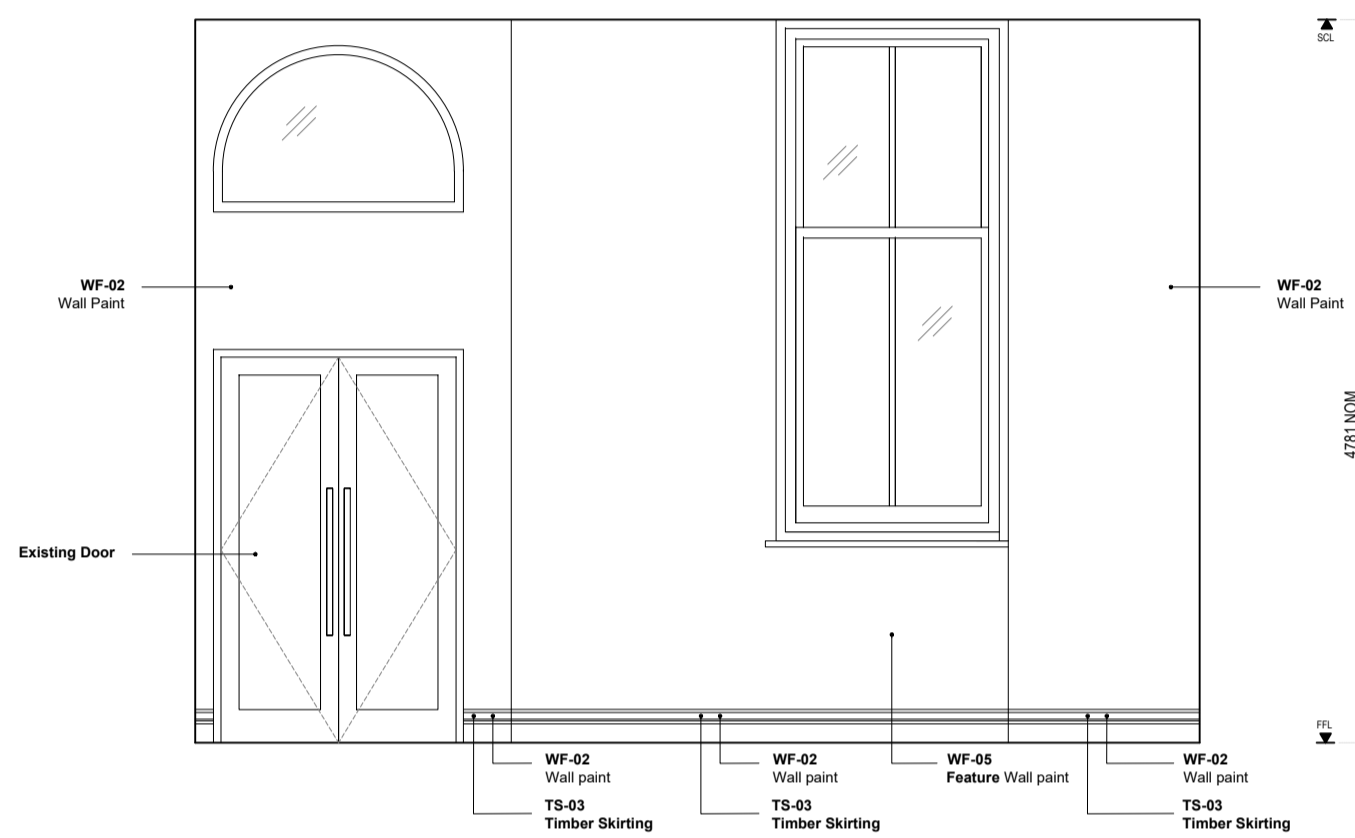
01 Proposed 203 Reception Elevation 1 1:50
