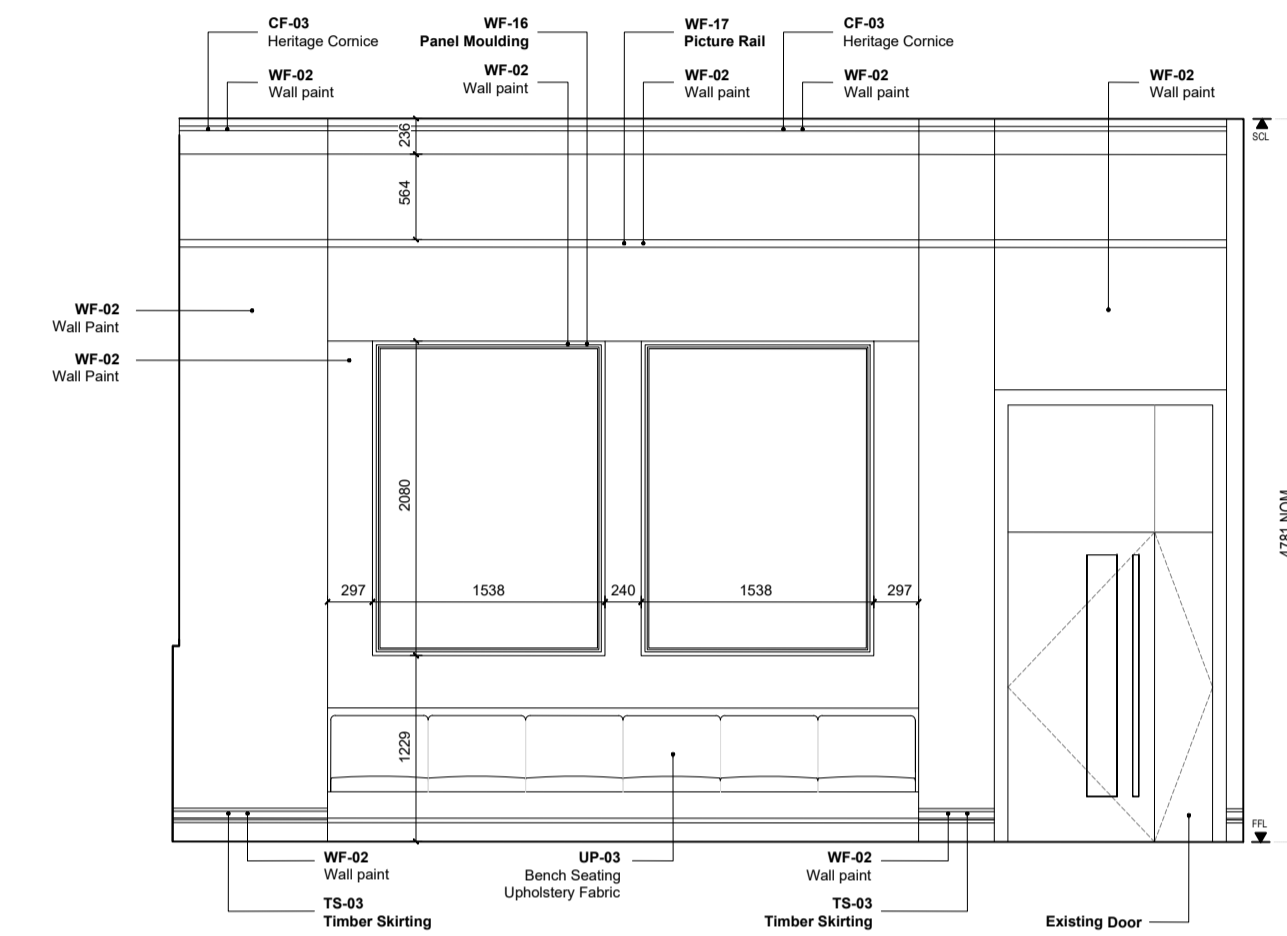
02 Proposed 203 Reception Elevation 2 1:50
