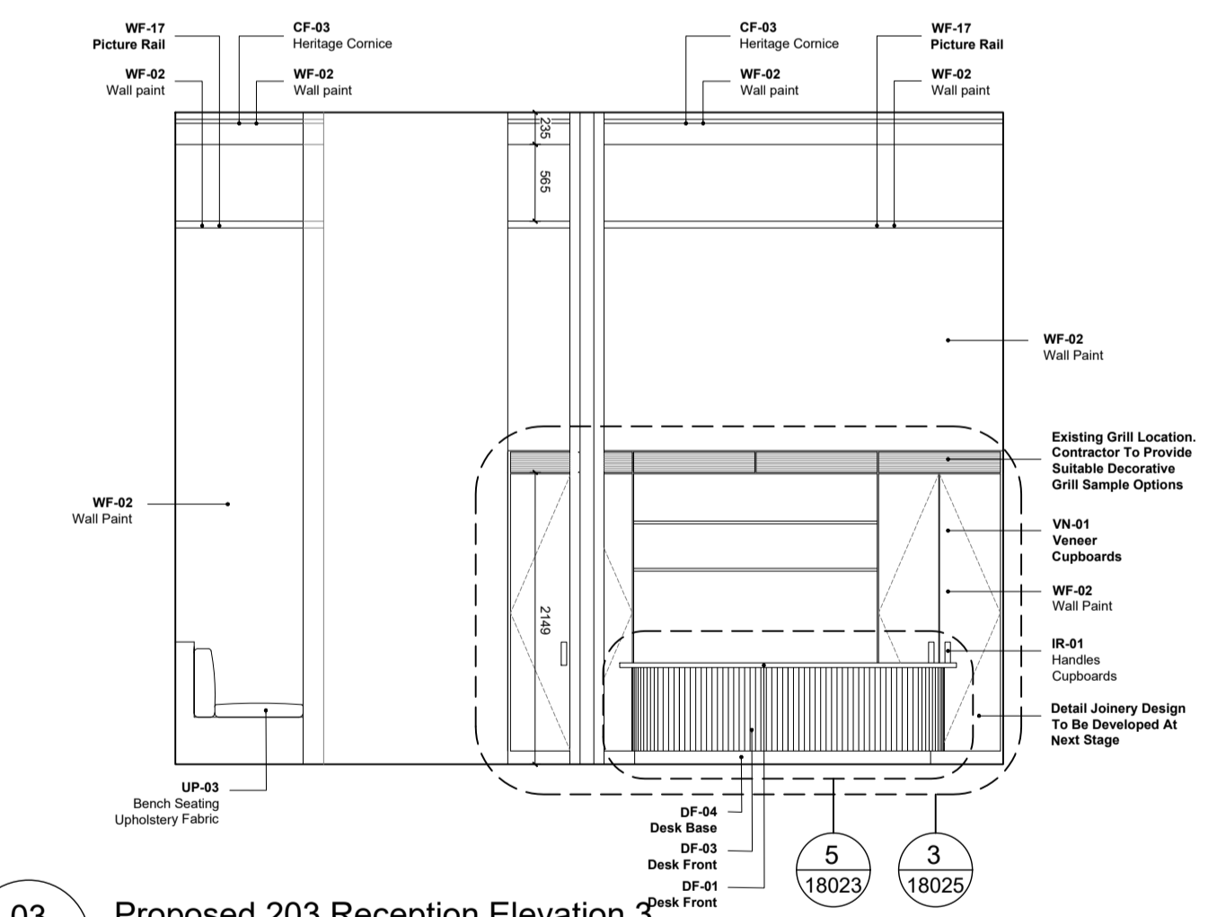
03 Proposed 203 Reception Elevation 3 1:50
