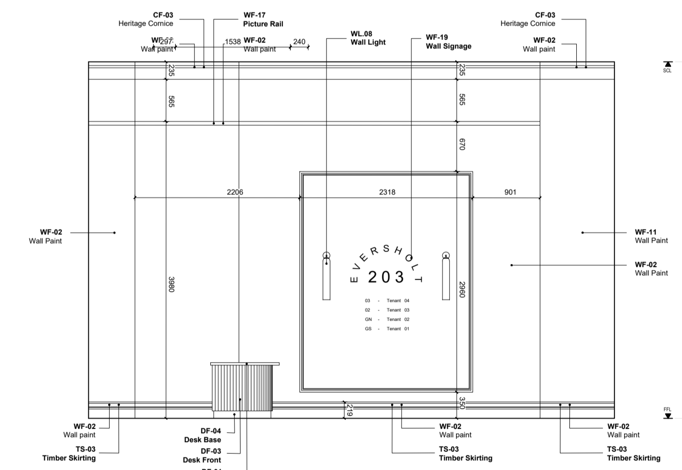
04 Proposed 203 Reception Elevation 4 1:50
