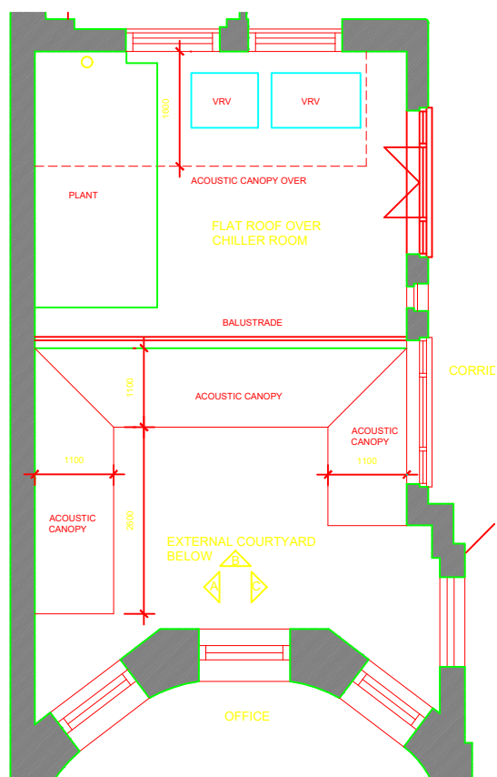
PART GROUND FLOOR PLAN
