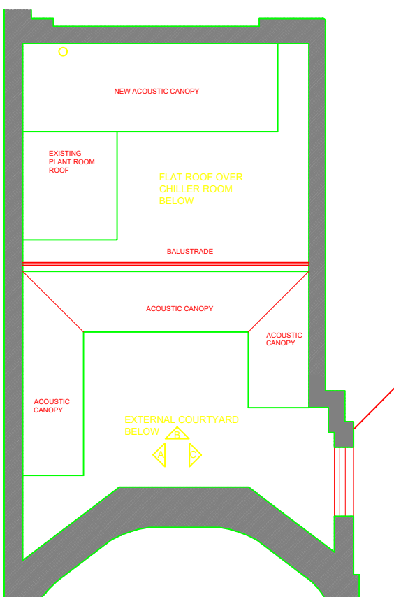
PLAN AT HIGH LEVEL
