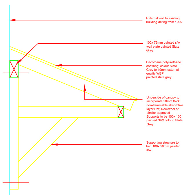
TYPICAL CANOPY DEATAILS 1:10
