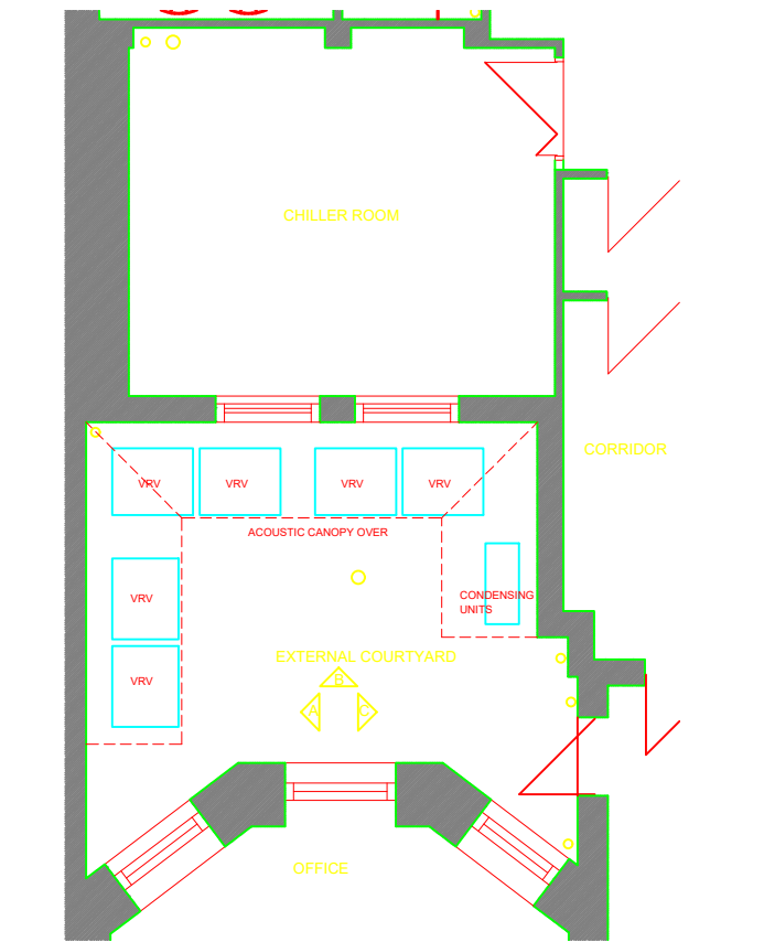
PART LOWER GROUND FLOOR PLAN
