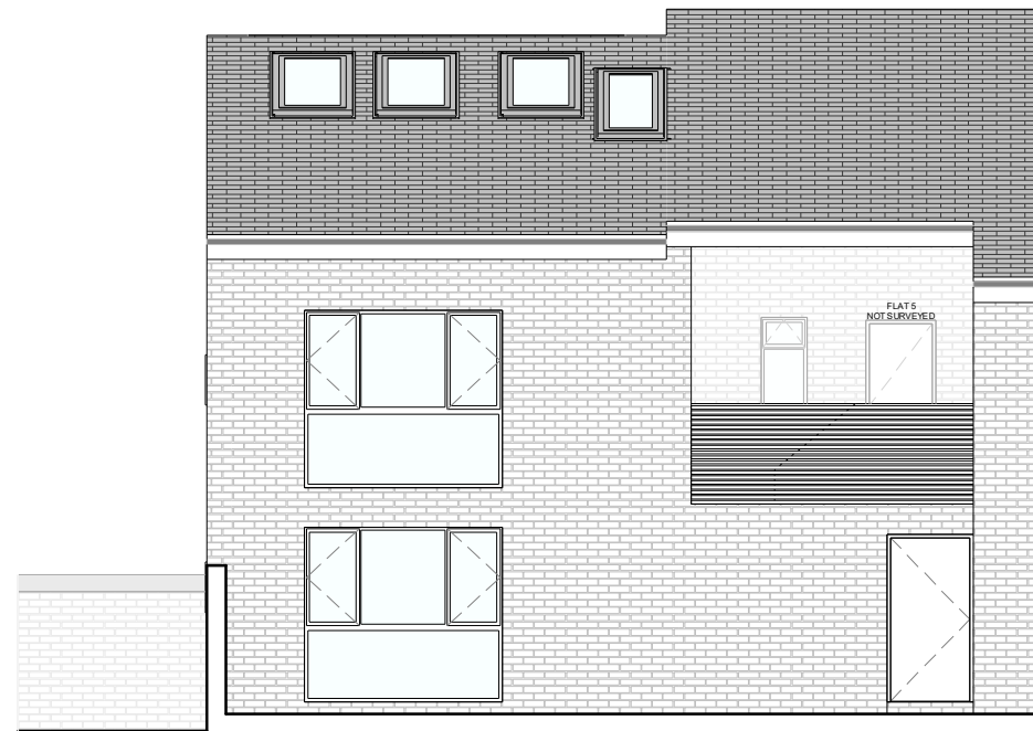
FRONT ELEVATION SCALE 1:100 @A3
