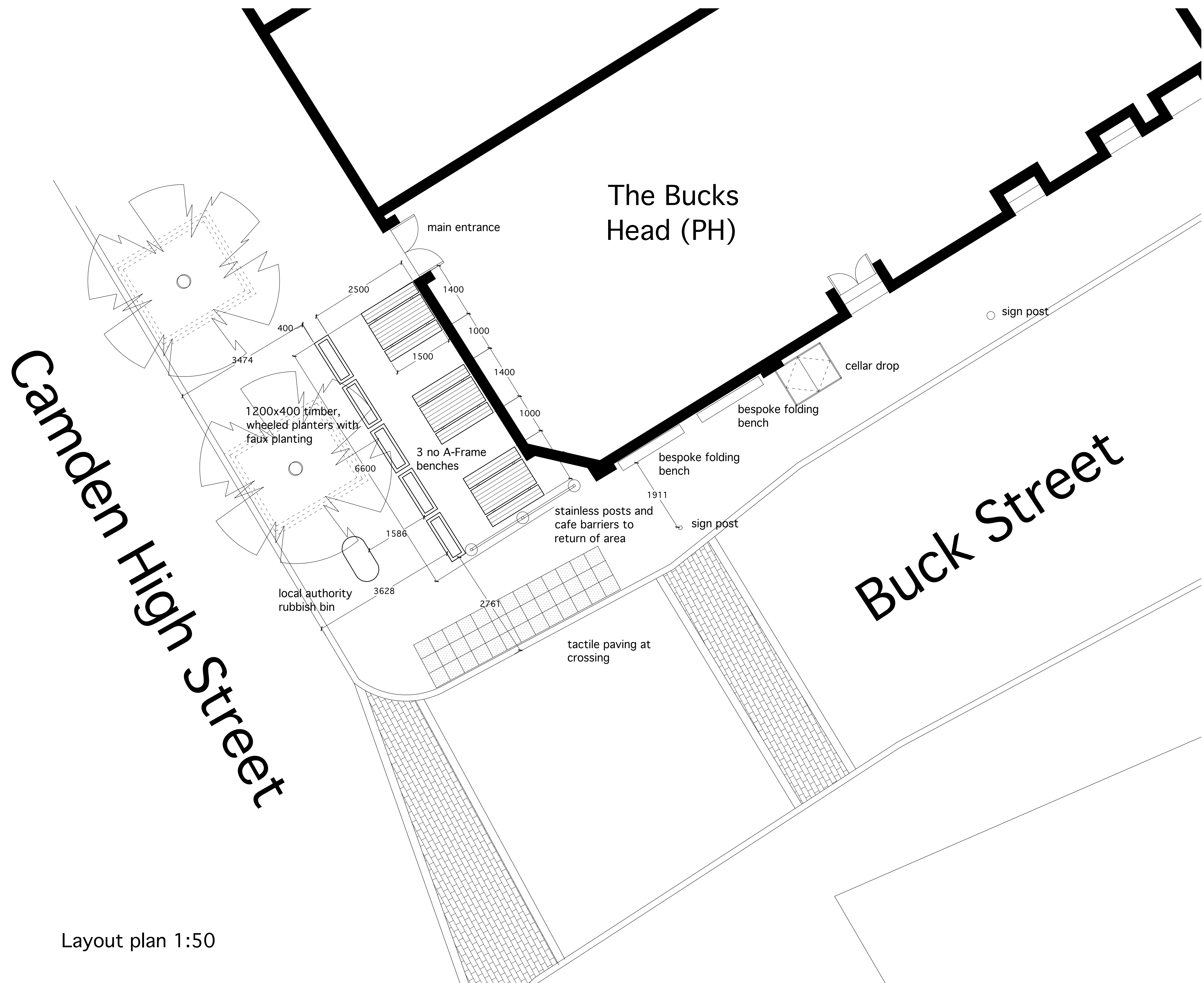
proposed side barriers - stainless steel posts with branded cafe barrier inserts - 1400mm long x 1000mm high
