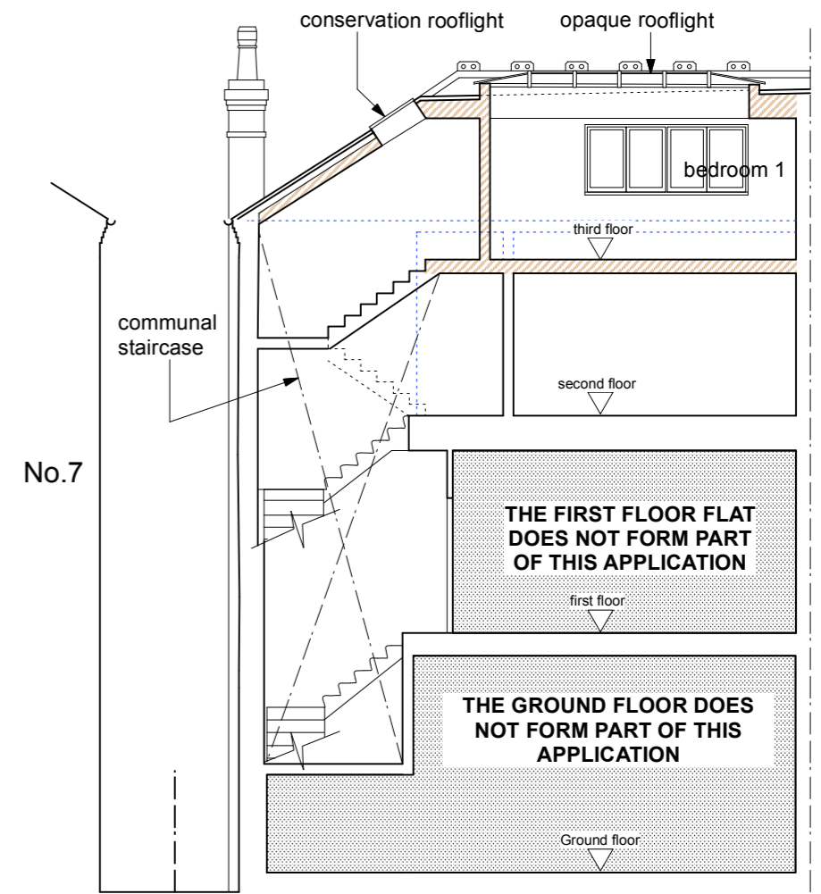
PROPOSED SECTION B-B
