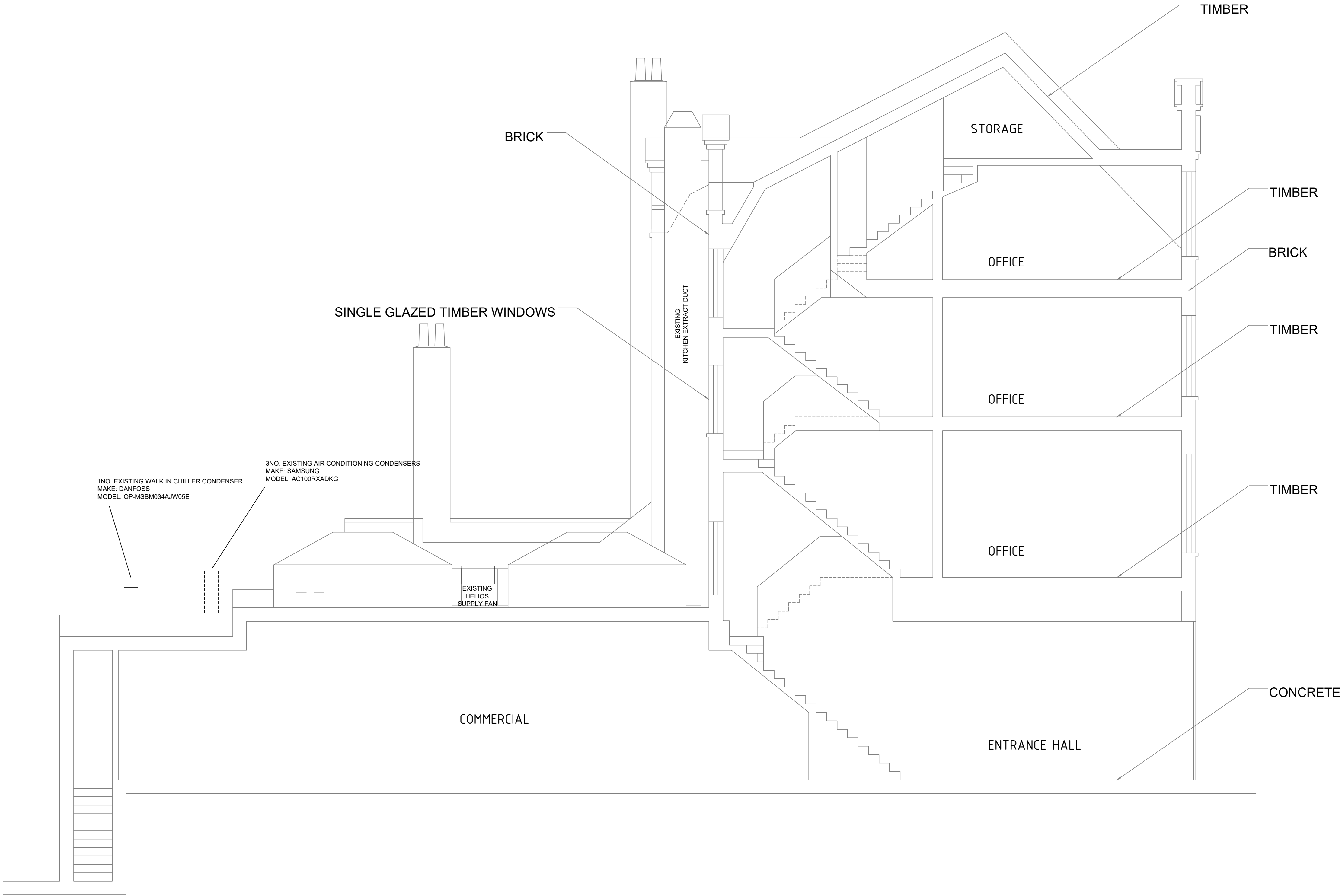
EXISTING SECTION A-A WITH KOJO HVAC PLANT
