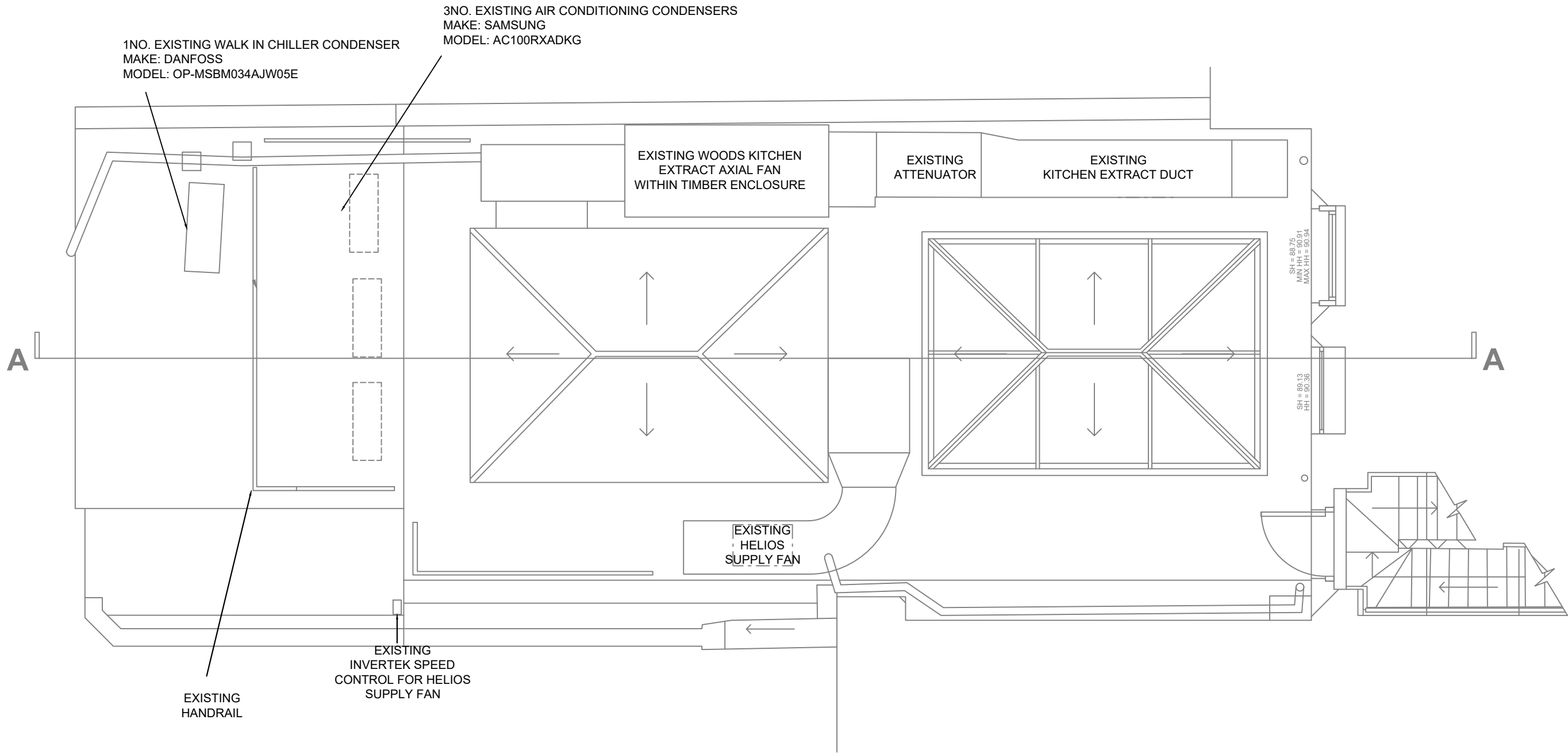
EXISTING REAR ROOF PLAN WITH KOJO HVAC PLANT
