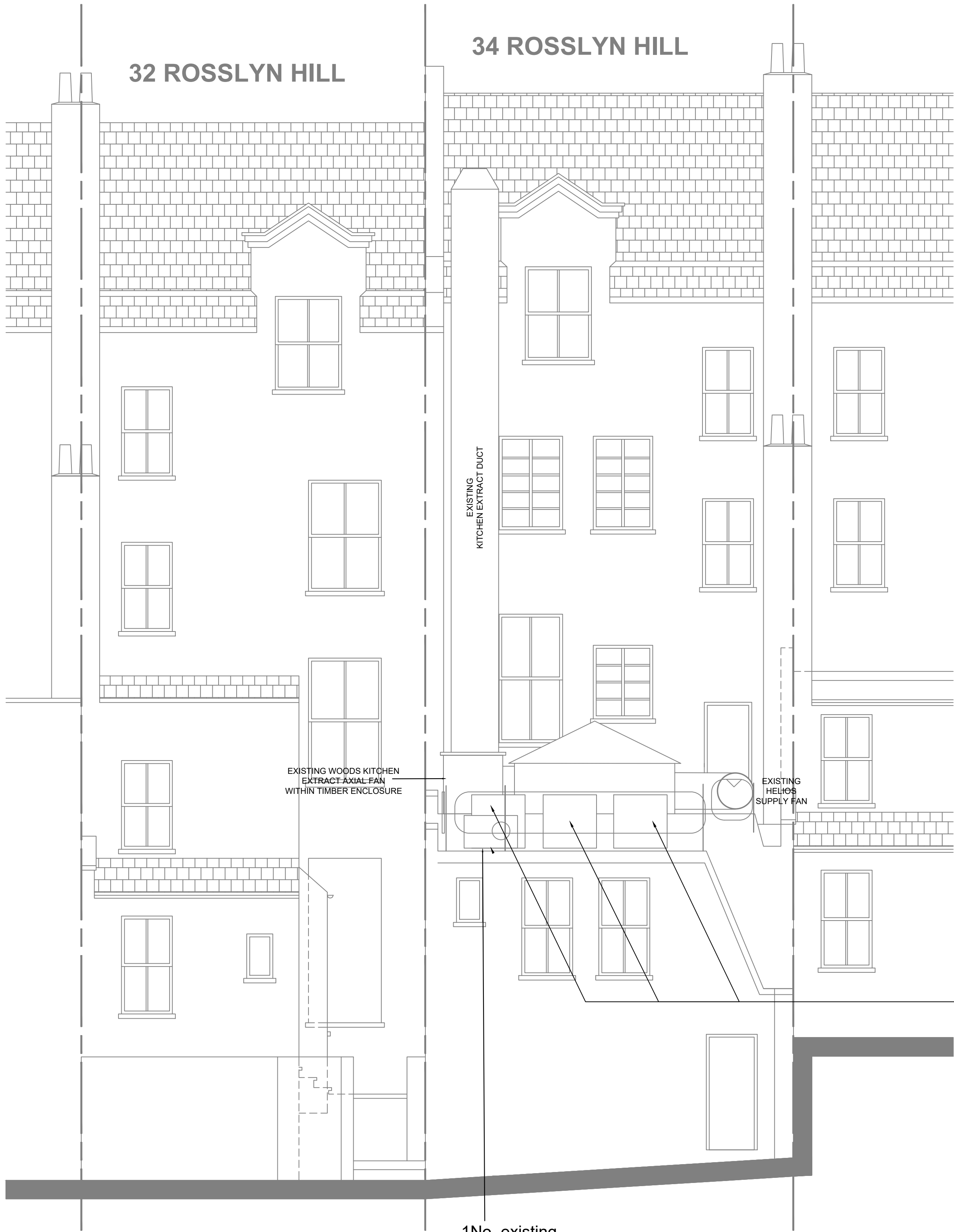
EXISTING REAR ELEVATION WITH KOJO HVAC PLANT
