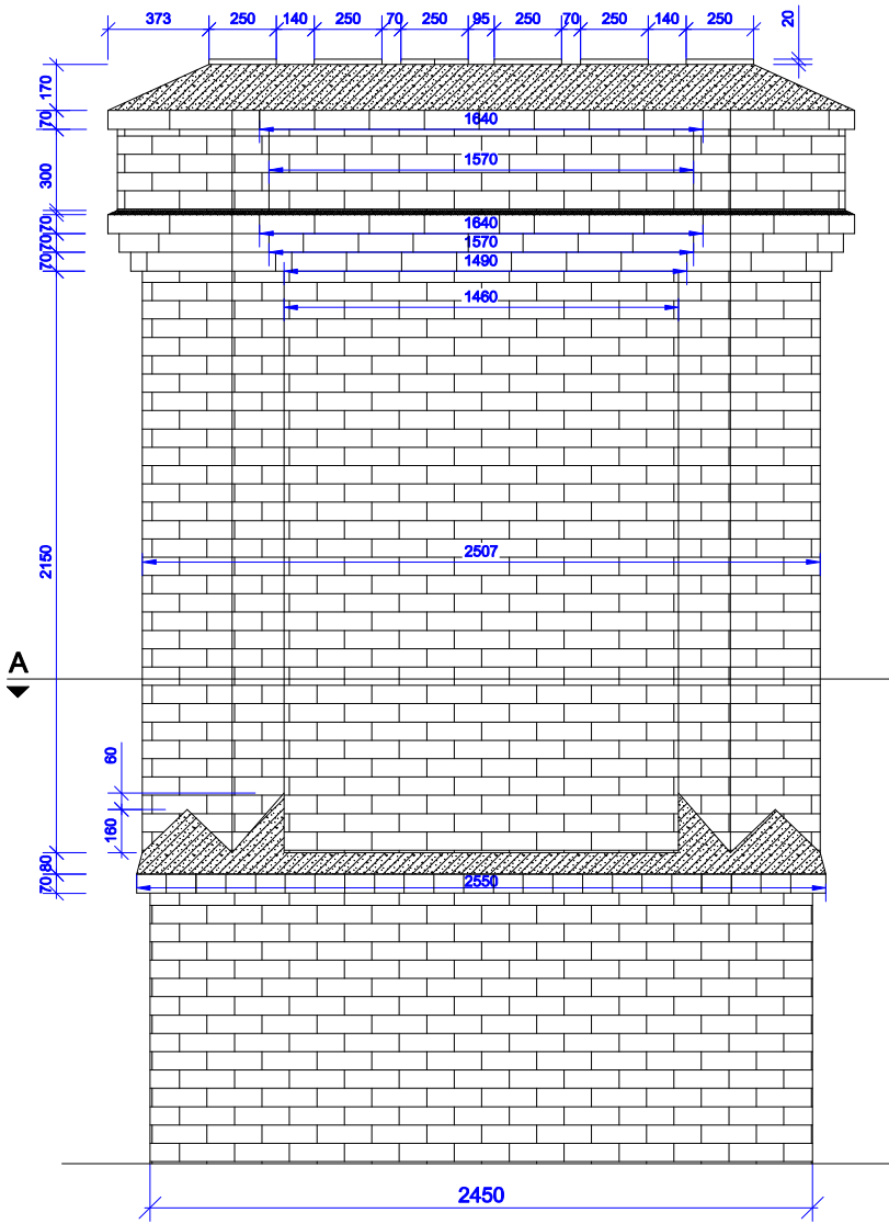
SIDE VIEW
