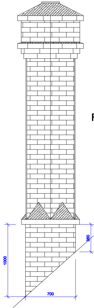
FRONT VIEW
