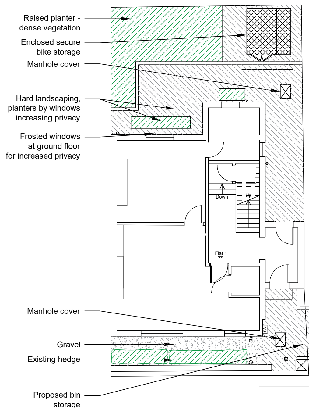
Proposed External Layout
