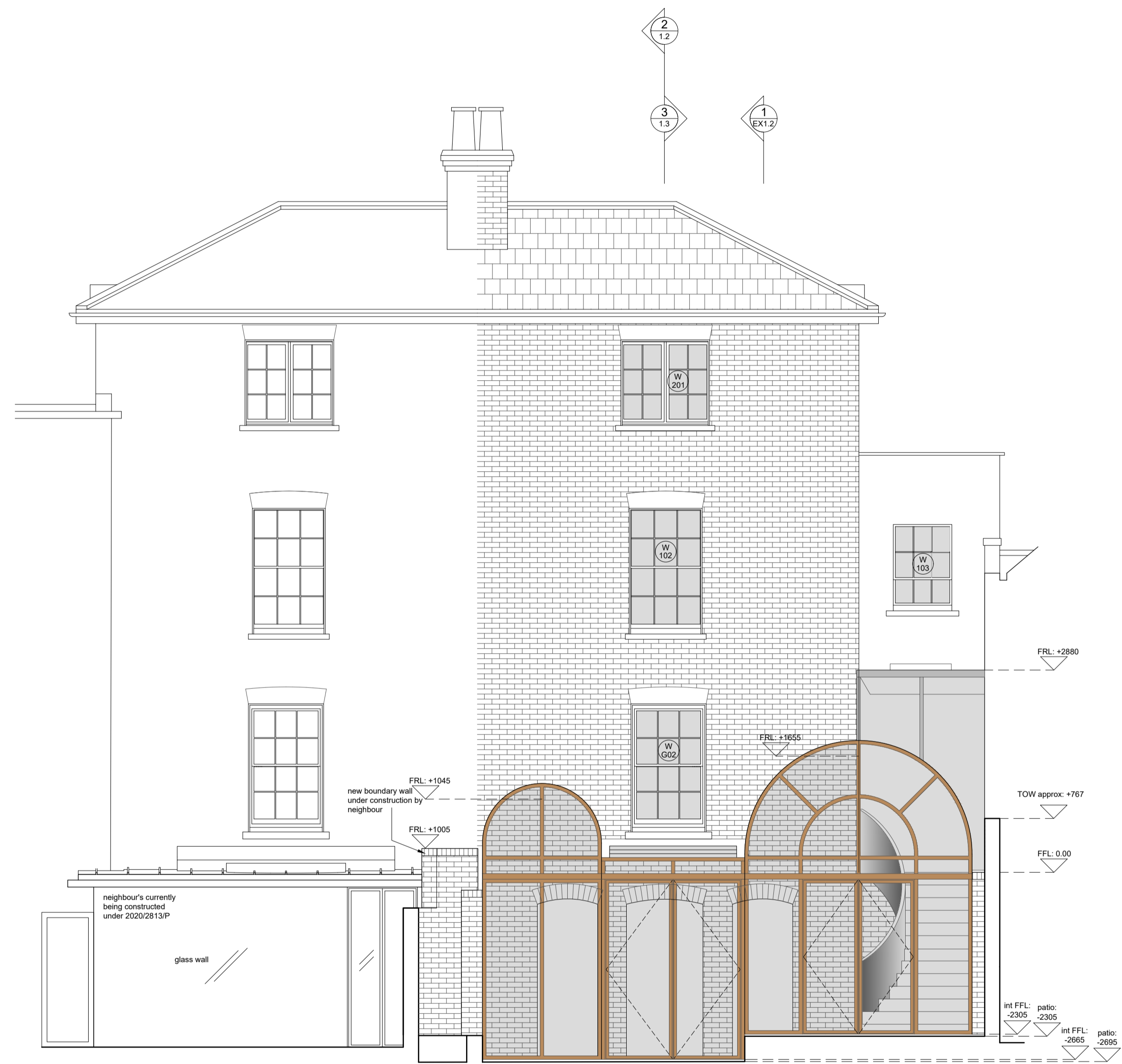
Rear Elevation as Proposed
