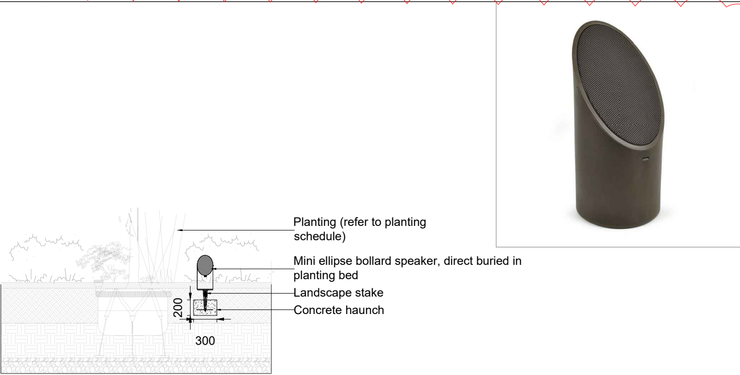
F8 Speakers MANUFACTURER: Coastal Source RANGE: 8.0 Mini Ellipse Bollard PRODUCT REFERENCE: EB82W6.5BN WEBSITE: www.coastalsource.com MATERIAL: Fiberglass Enclosure with Aluminum Grill FIXING: Surface/direct burial installation with stake and theft guard in planting beds. Drainage hole to be 25mm (min.) above ground.
