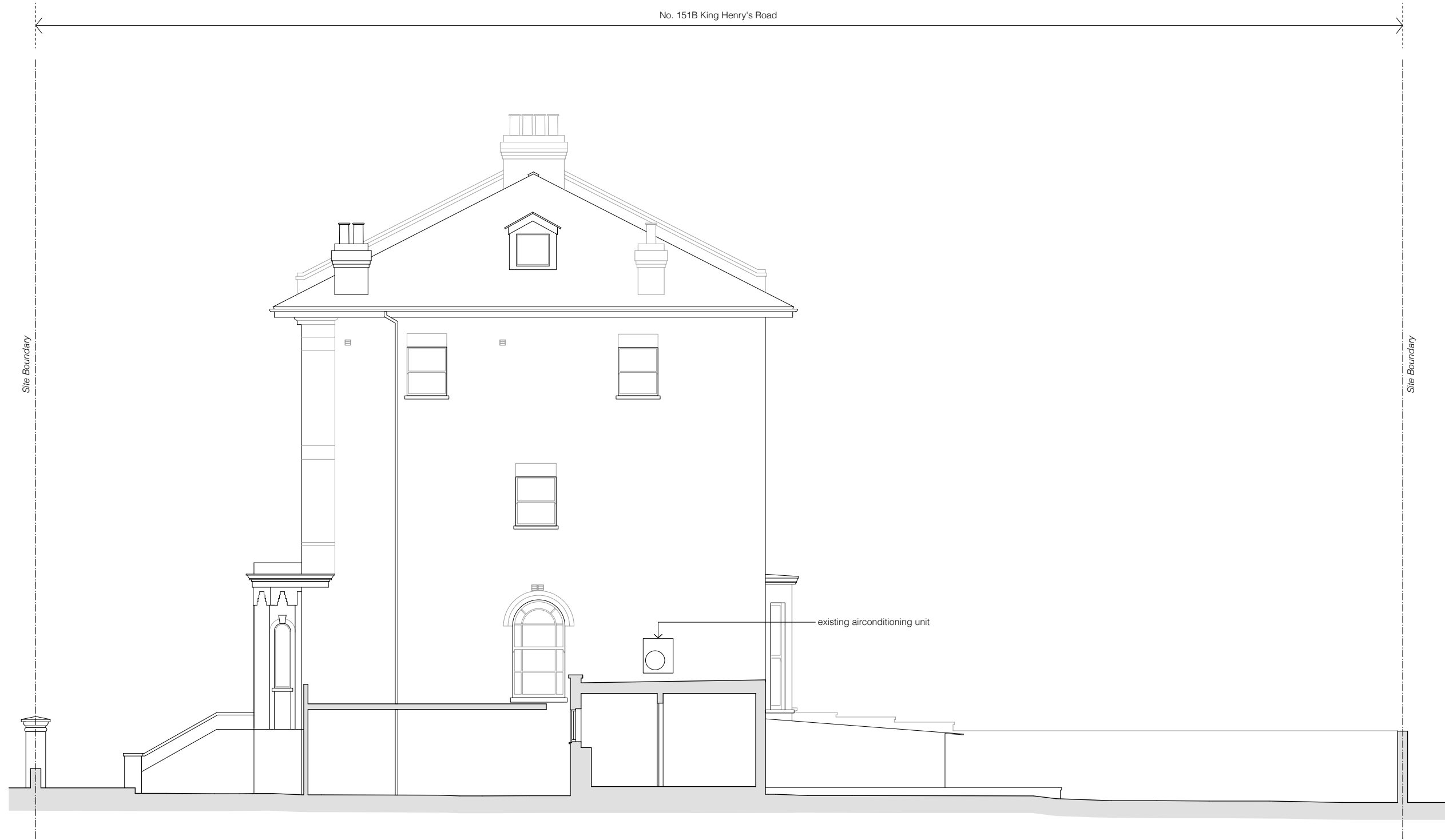
SIDE ELEVATION: EXISTING
