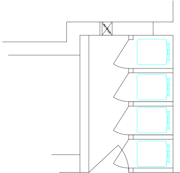
Existing - Plan
