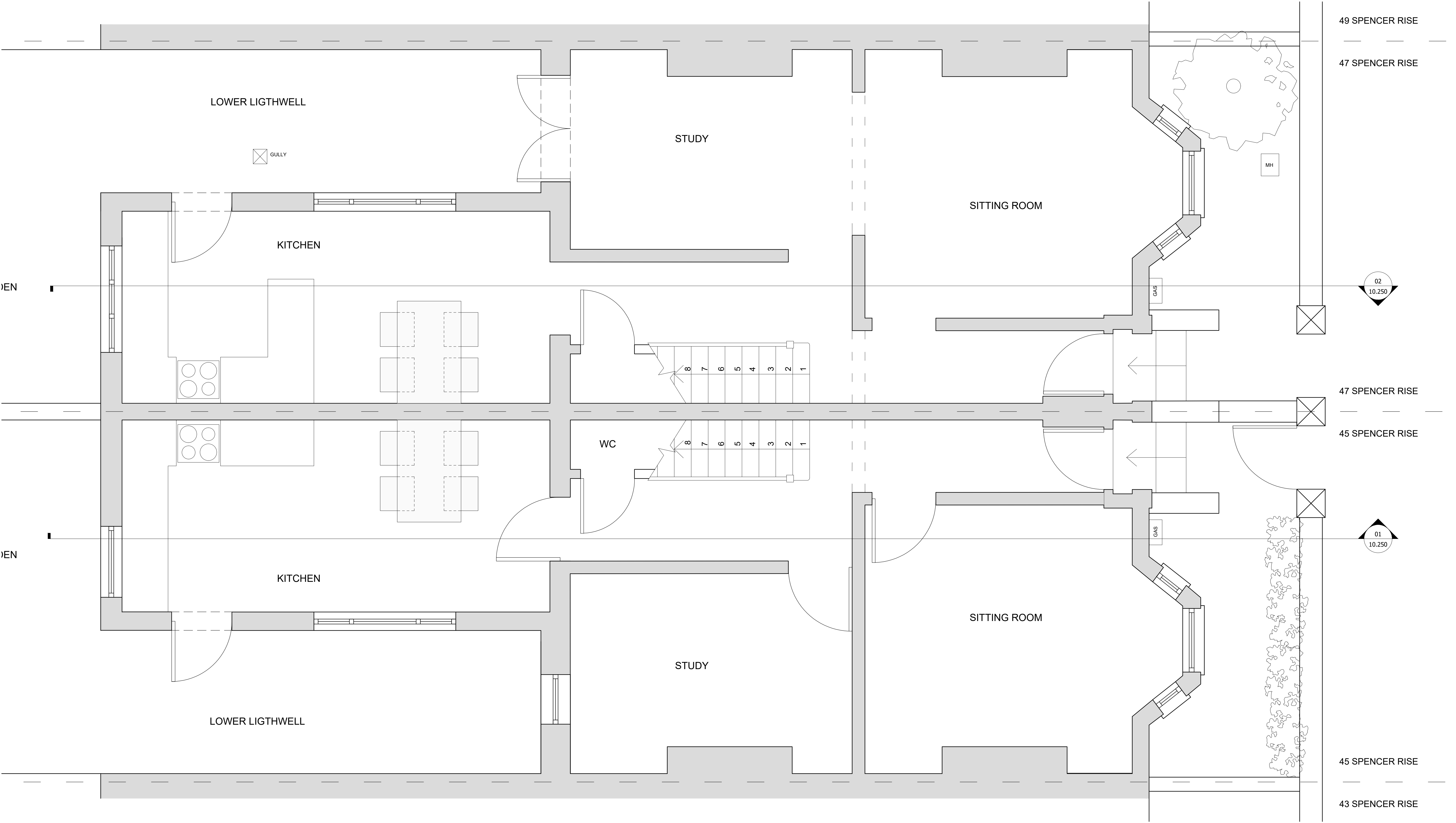
01 10.200 Existing Ground Floor Plan 1:25@A1, 1:50@A3
