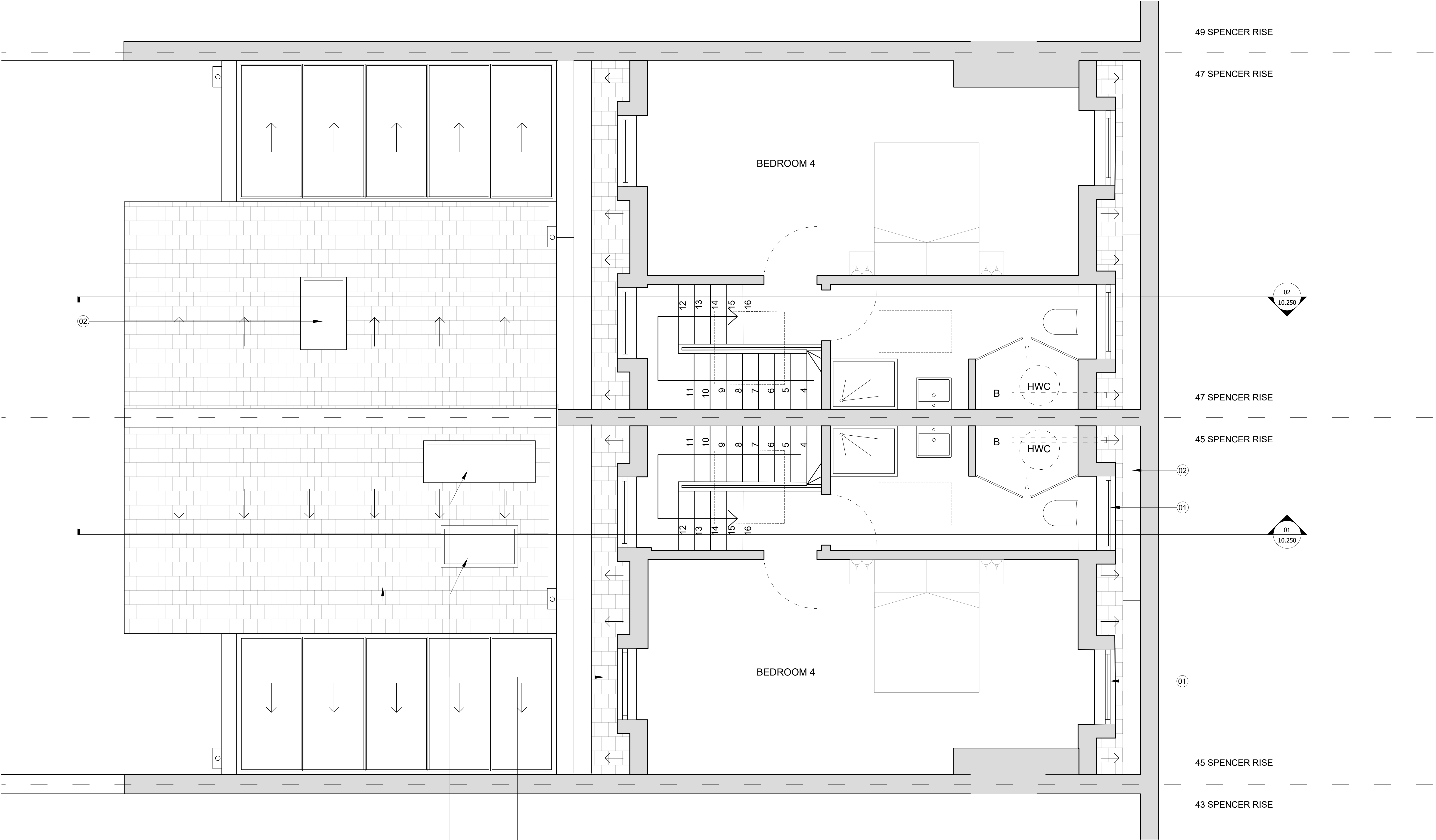
01 10.202 Proposed Mansard Floor Plan 1:25@A1, 1:50@A3
