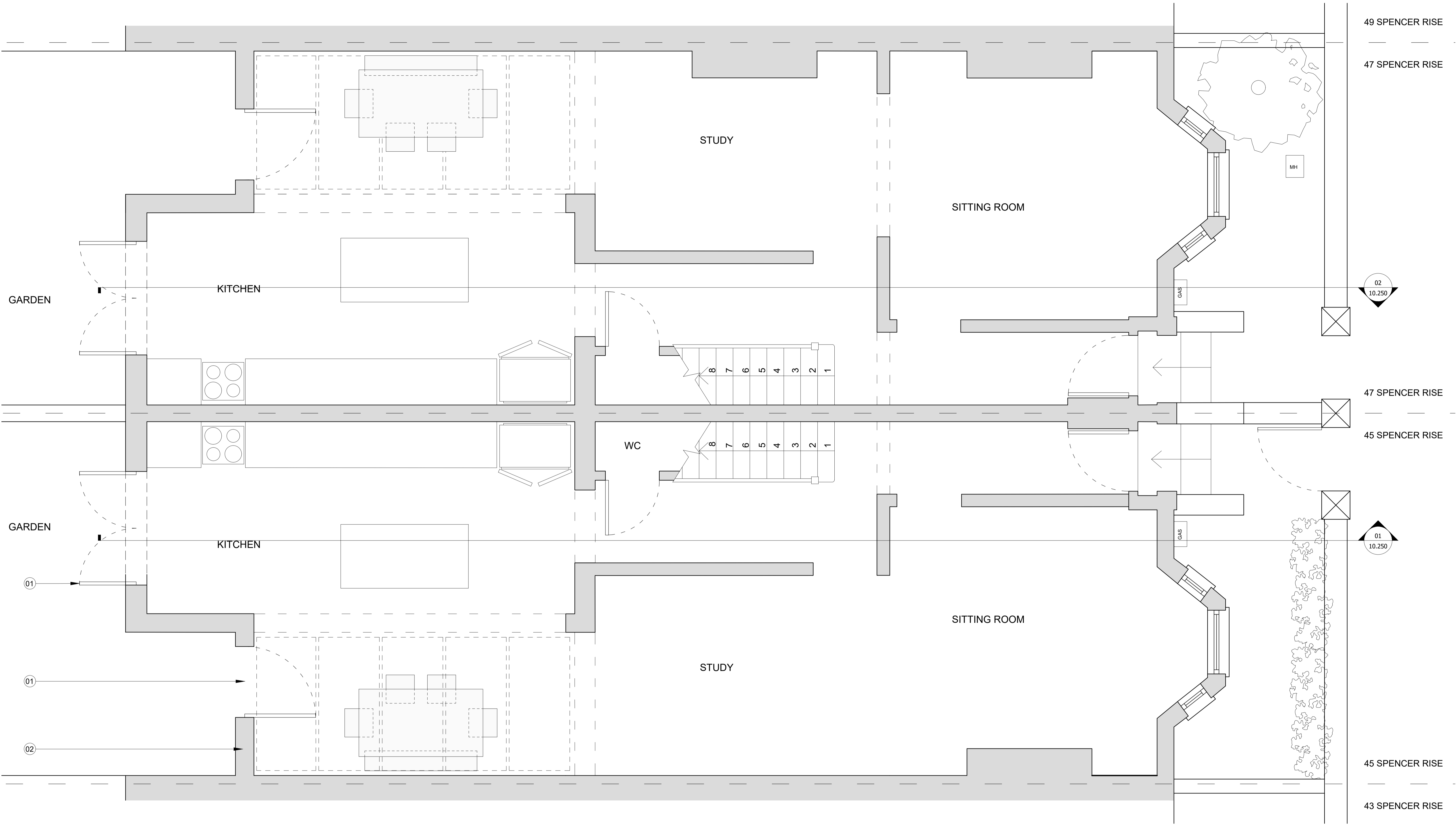
01 20.200 Proposed Ground Floor Plan 1:25@A1, 1:50@A3
