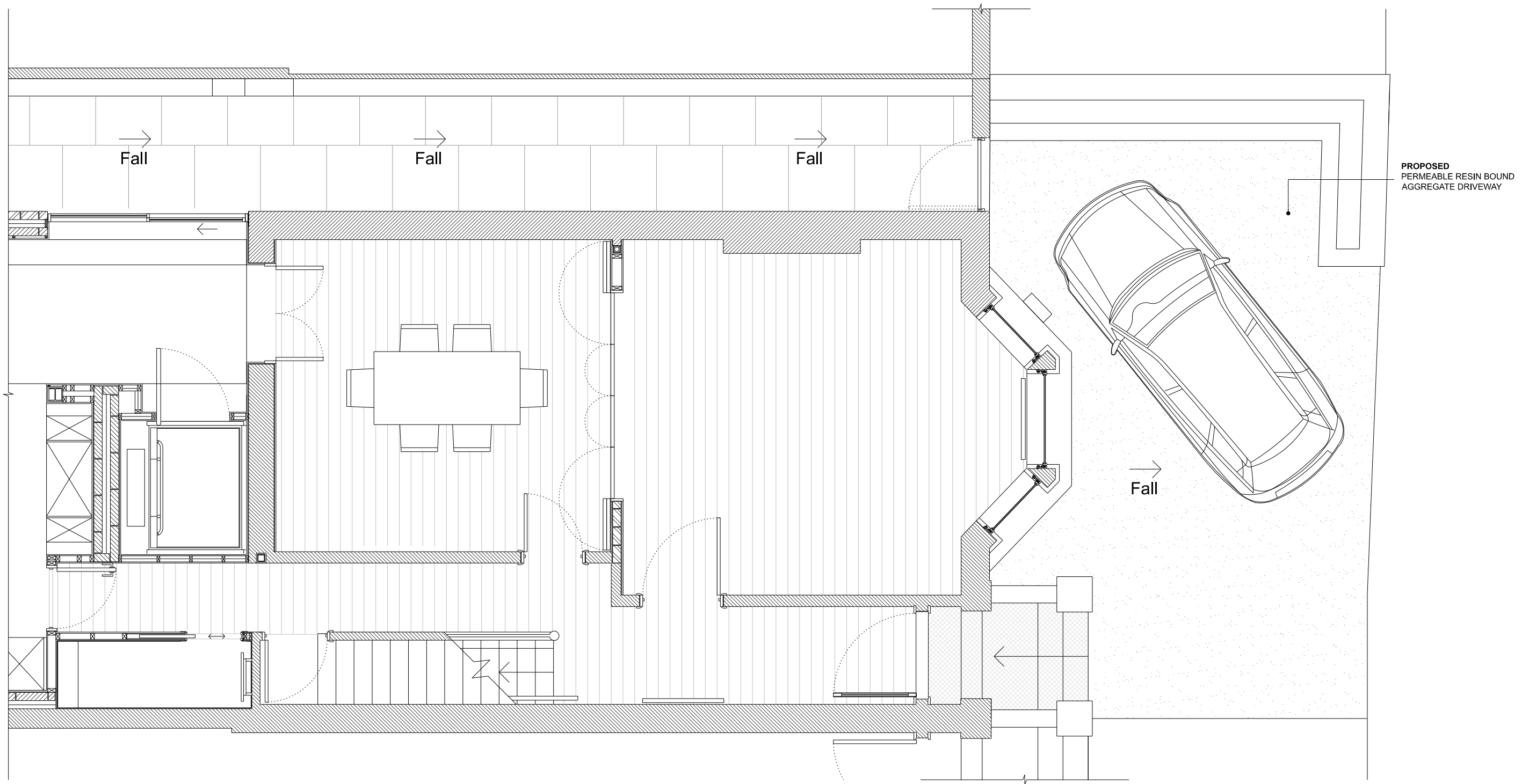
01 PROPOSED PART GROUND FLOOR PLAN 1:50 @A3
