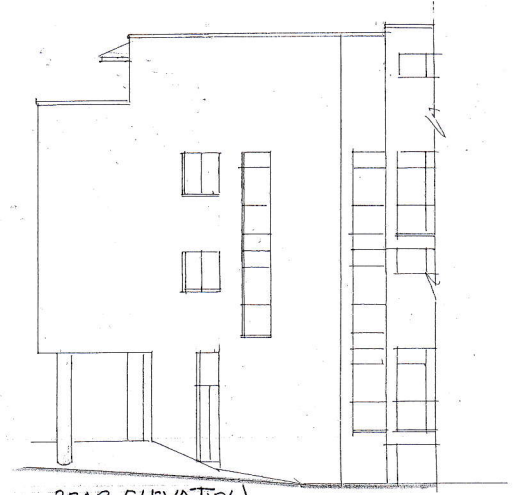
REAR ELEVATION
