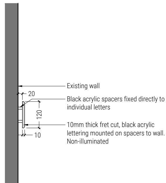
Section Through 'Regent's Canal Information Centre' Acrylic Lettering
