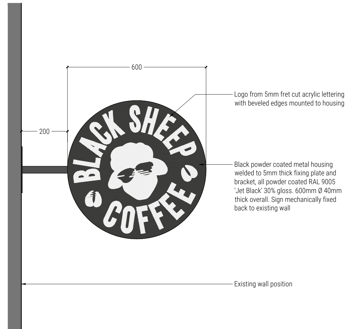
Projecting Sign Side Elevation
