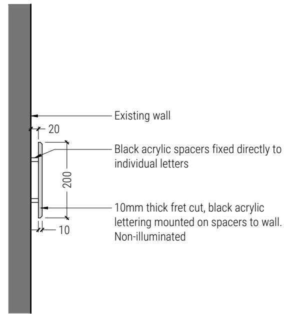
Section Through 'Black Sheep Coffee' Acrylic Lettering
