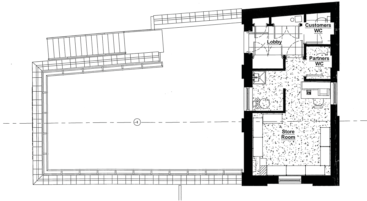
Proposed First Floor Layout
