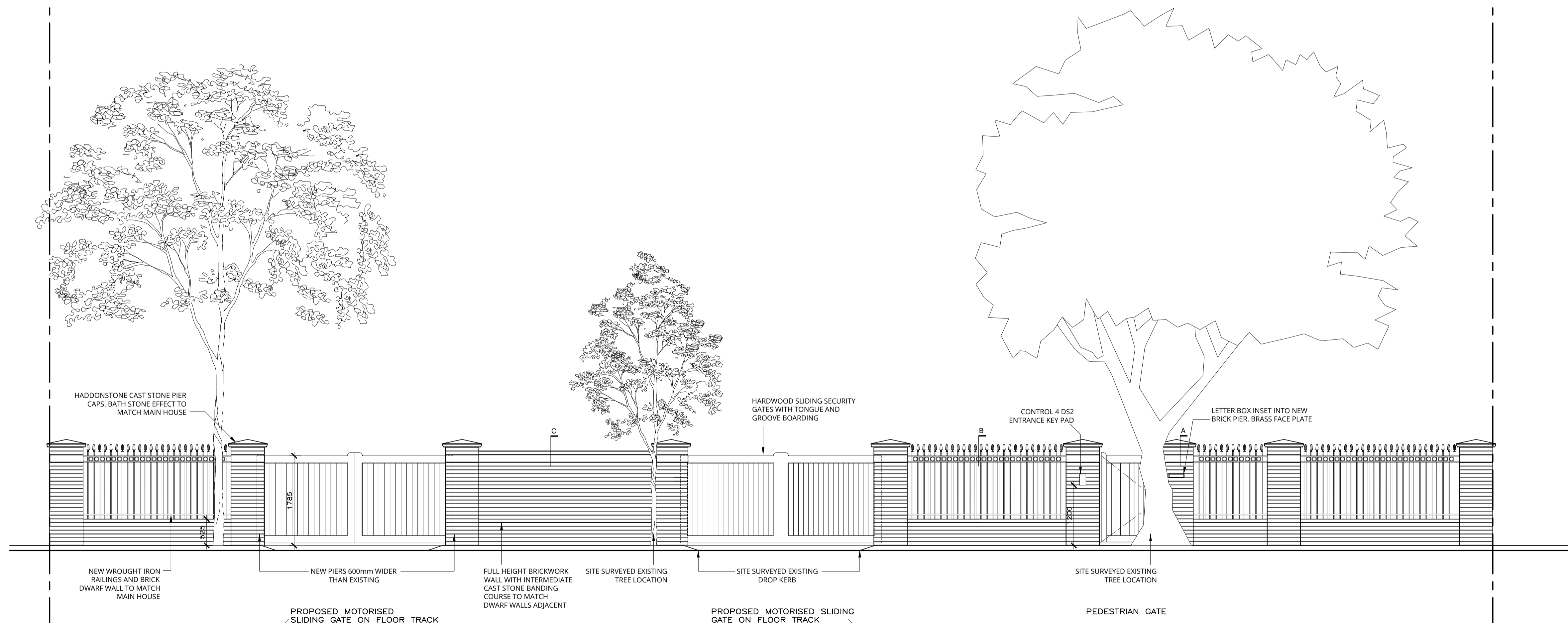
PROPOSED FRONT ENTRANCE GATES AND WALL ELEVATION
