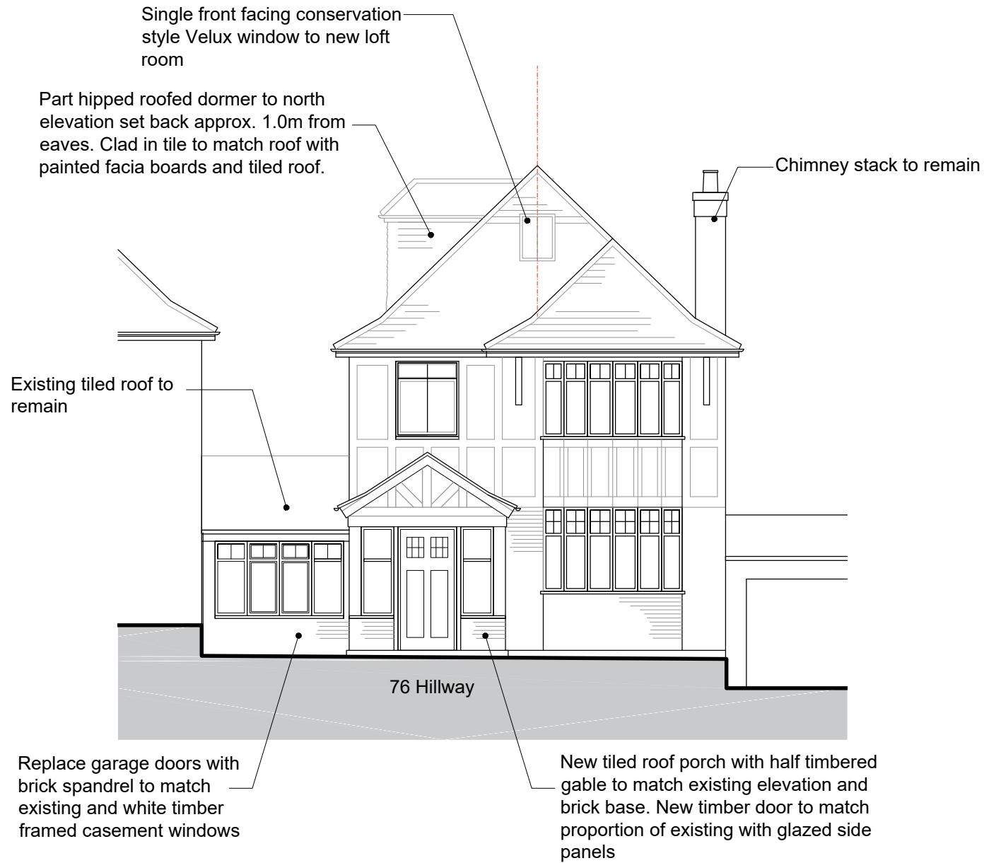
1. PROPOSED FRONT ELEVATION
