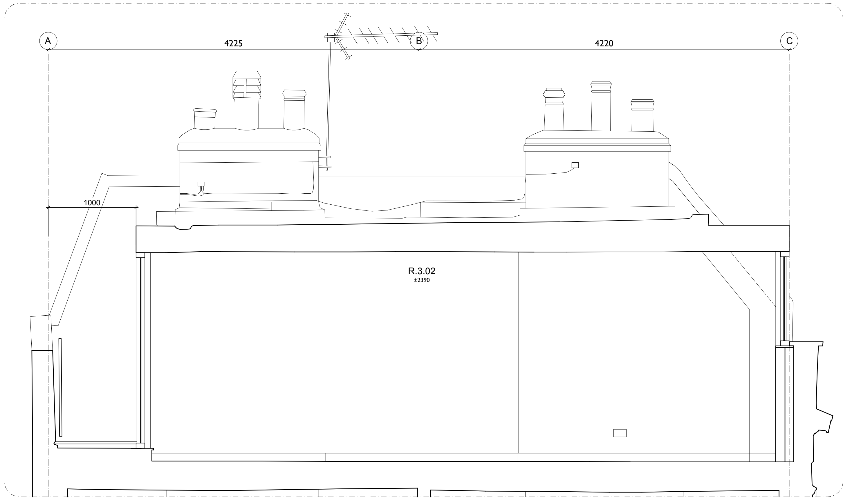
SECTION A
