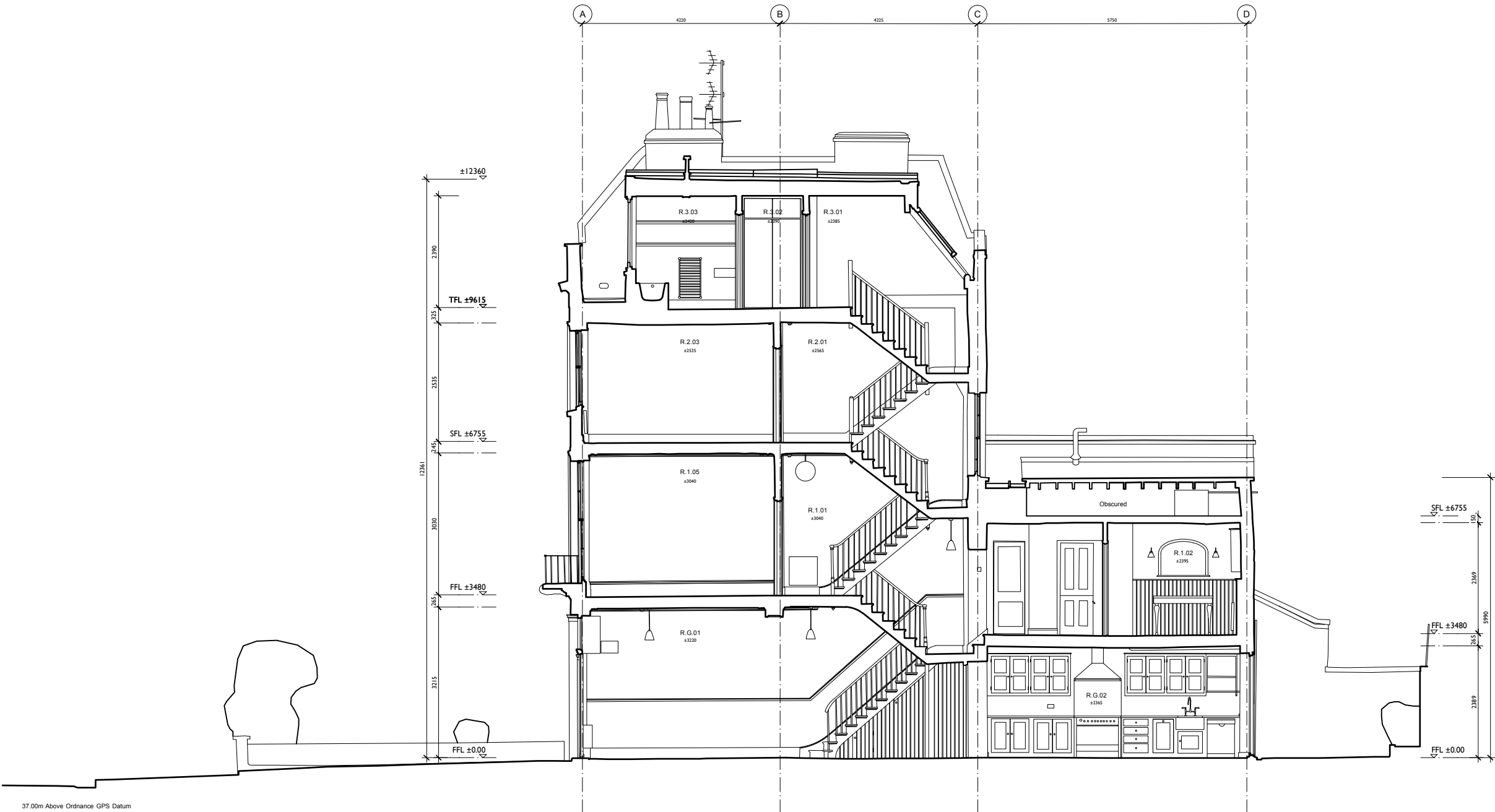
SECTION B
