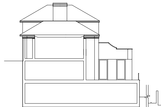
4. Proposed Section B-B
