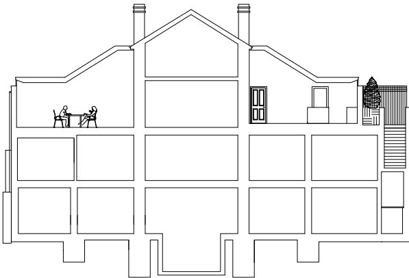
4. Proposed Section AA
