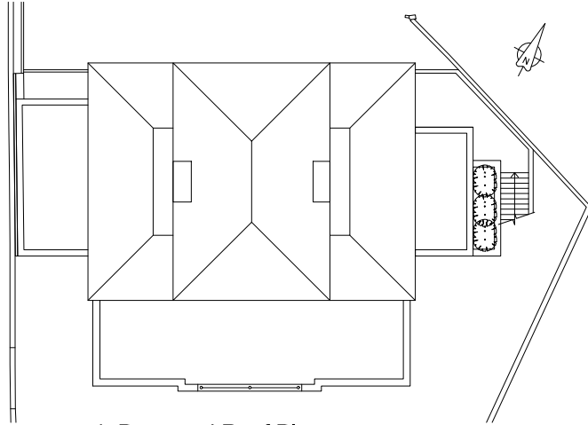
4. Proposed Roof Plan
