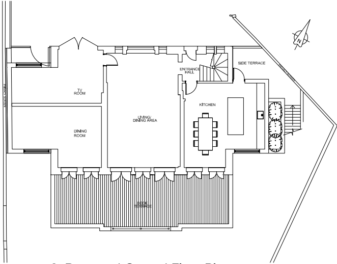
2. Proposed Ground Floor Plan
