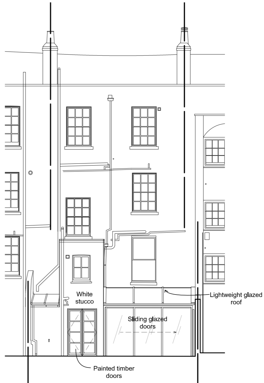
REAR ELEVATION
