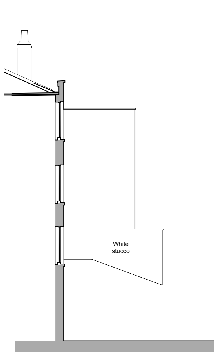
LEFT REAR ELEVATION
