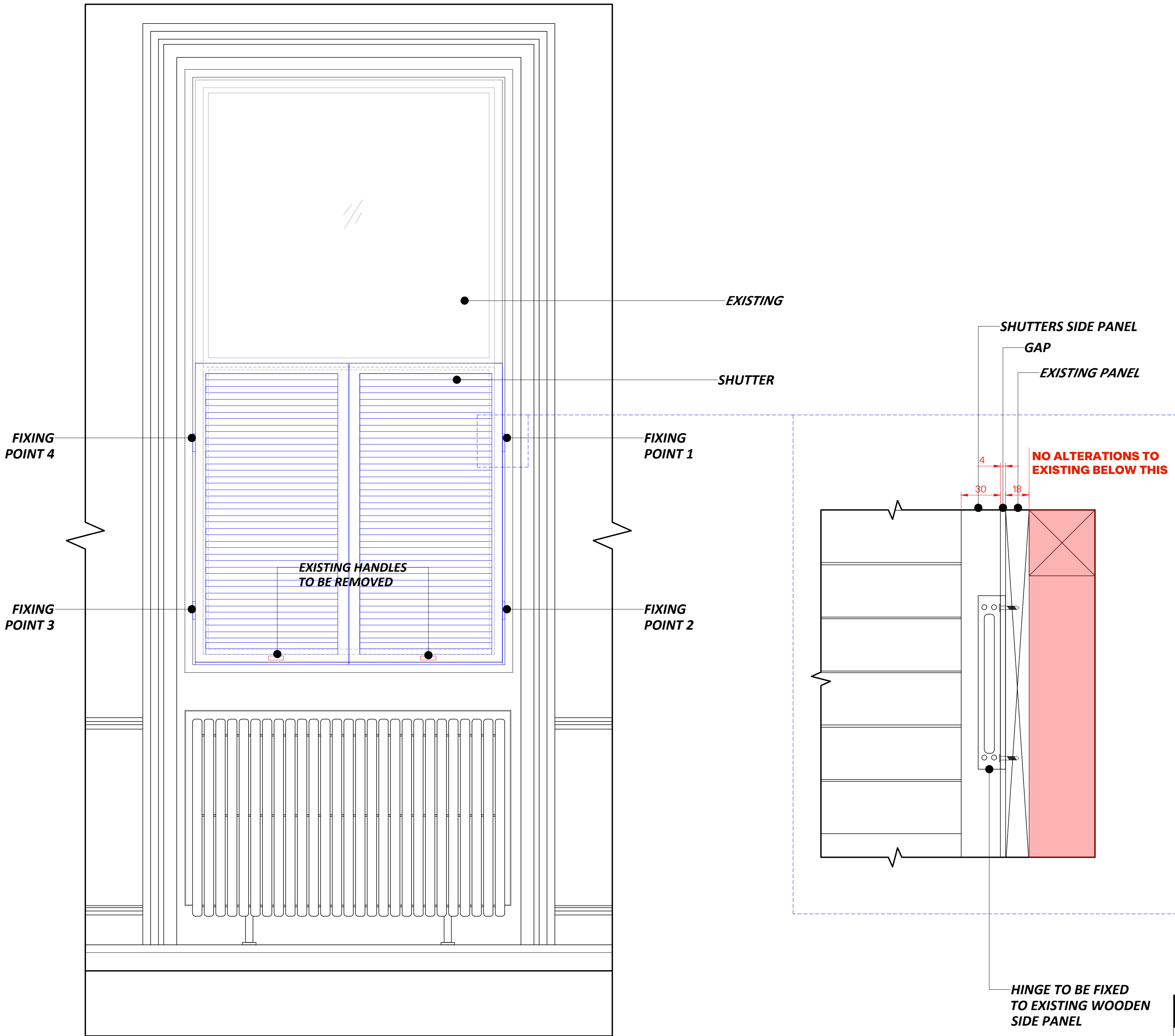
02 WINDOW - SHUTTER TYPICAL ELEVATION Scale: 1:10@A1
