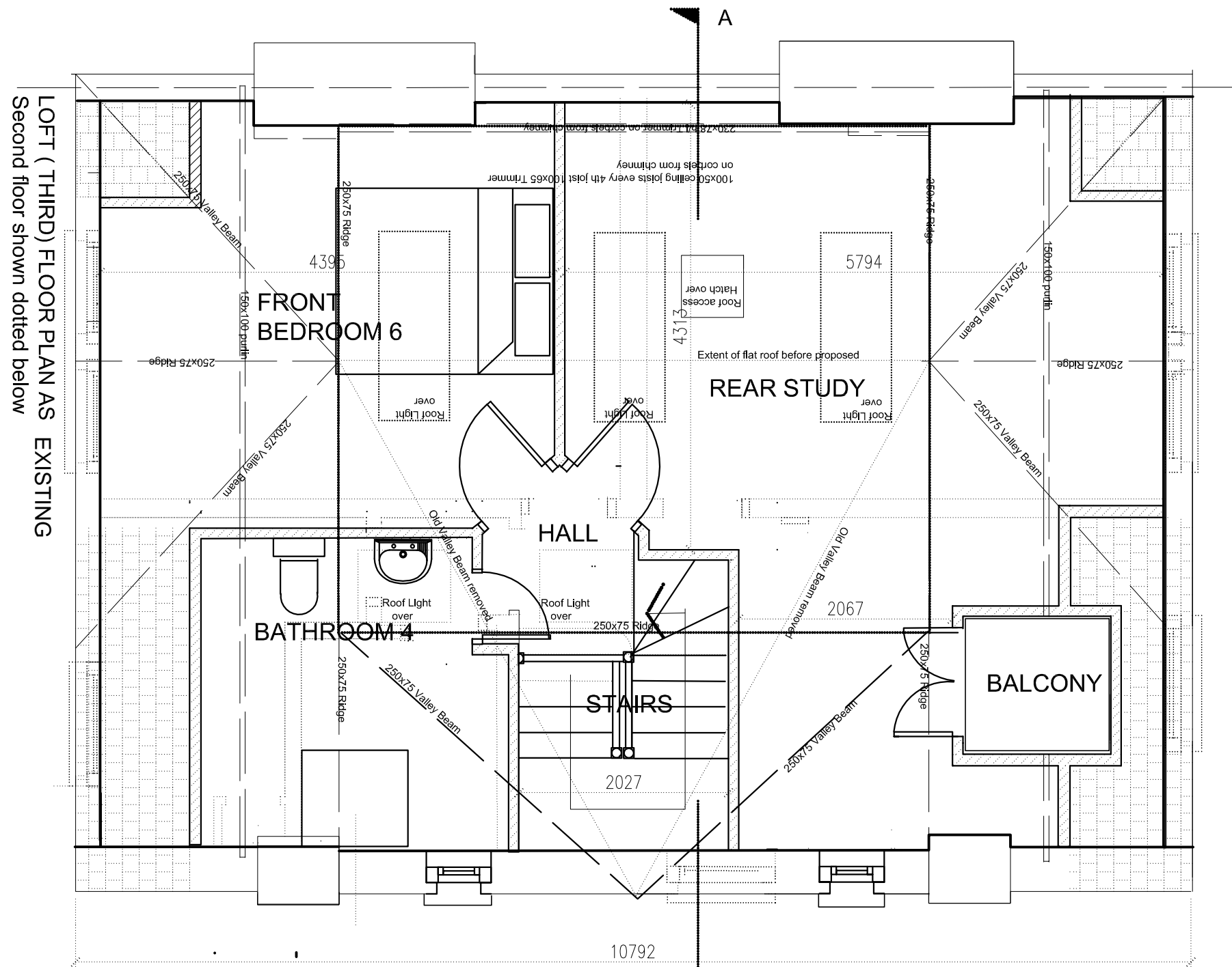
LOFT (THIRD) FLOOR PLAN AS EXISTING Second floor shown dotted below
