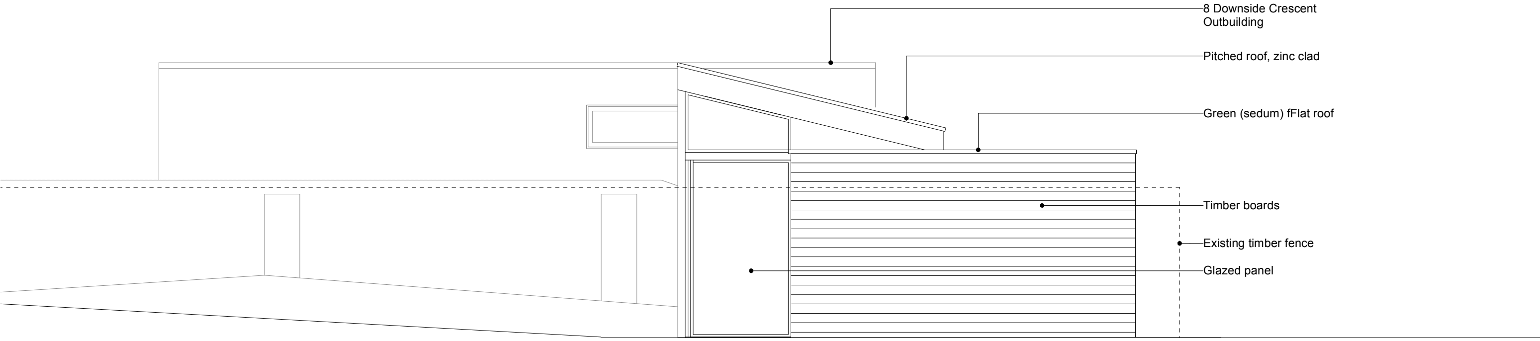
Side Elevation
