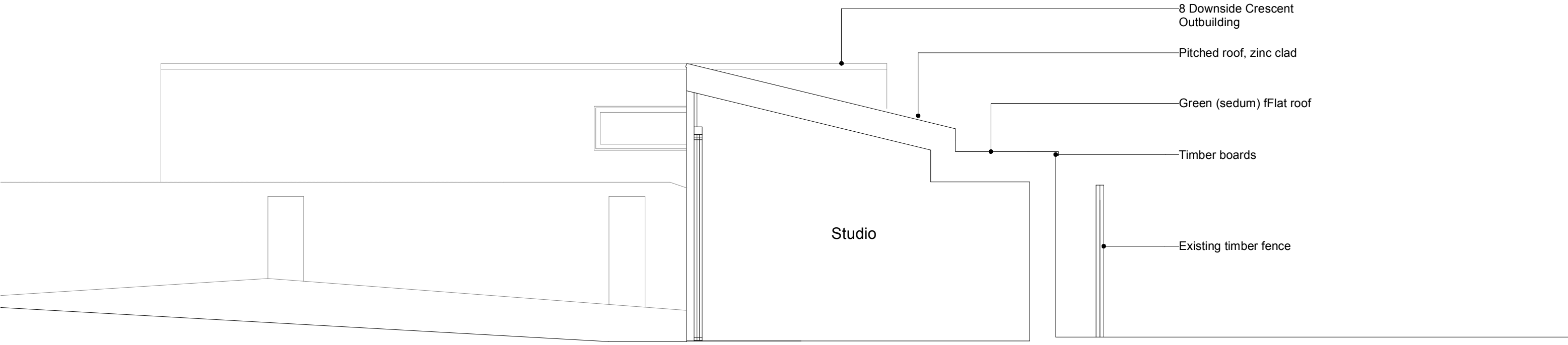
Section BB
