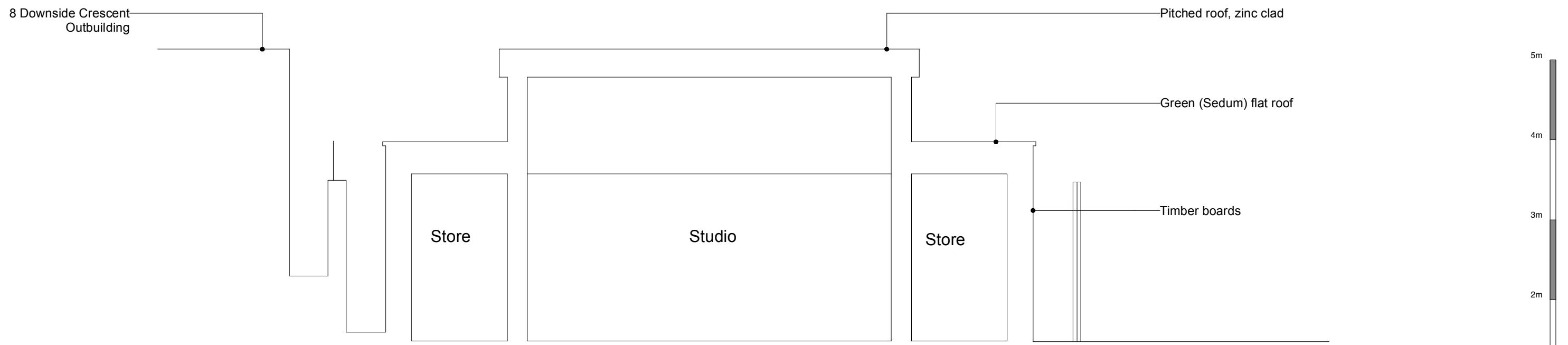
Section AA
