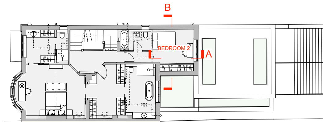
1 First Floor Key Plan Scale: 1:200 @ A3
