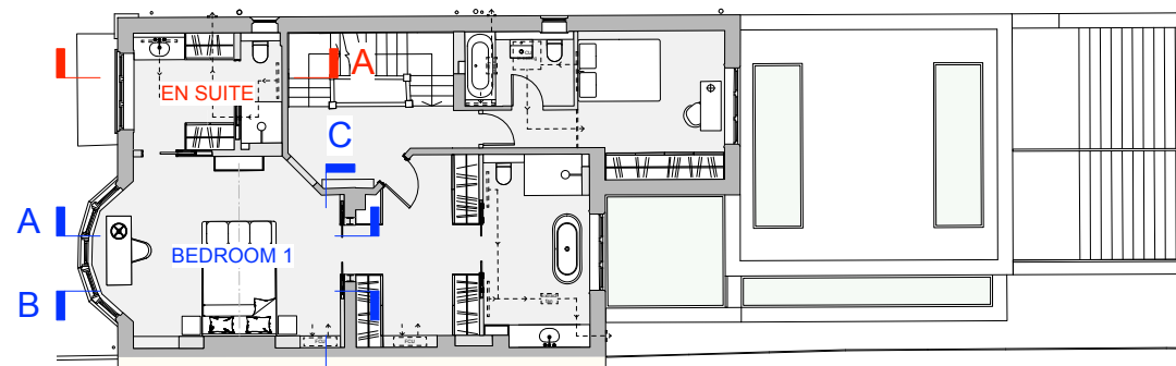
1 First Floor Key Plan Scale: 1:200 @ A3
