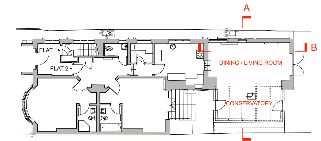
1 Ground Floor Key Plan Scale: 1:200 @ A3
