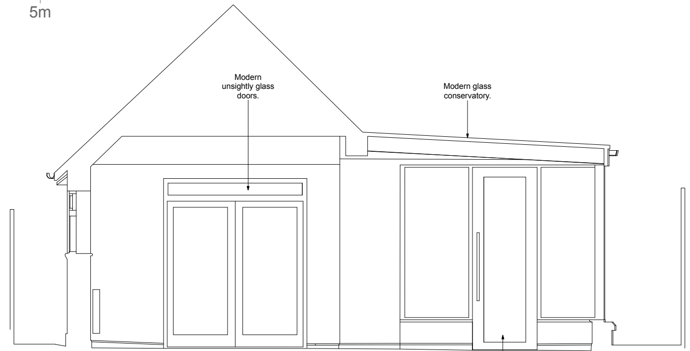
A Dining / Living / Conservatory - Elevation A Scale: 1:50 @ A3
