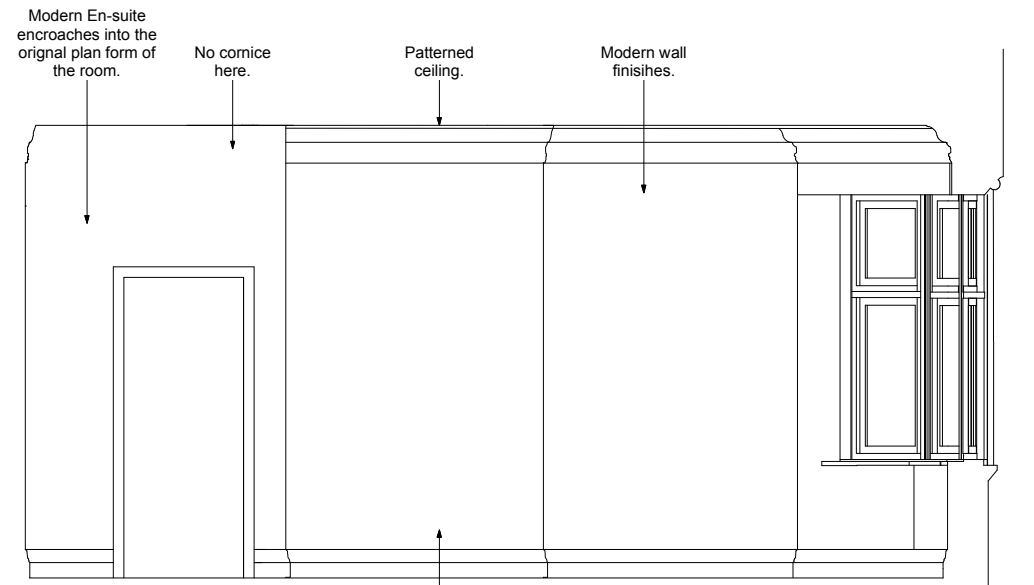
B Bedroom 1 - Elevation B Scale: 1:50 @ A3 Only one side of chimney breast is visible.
