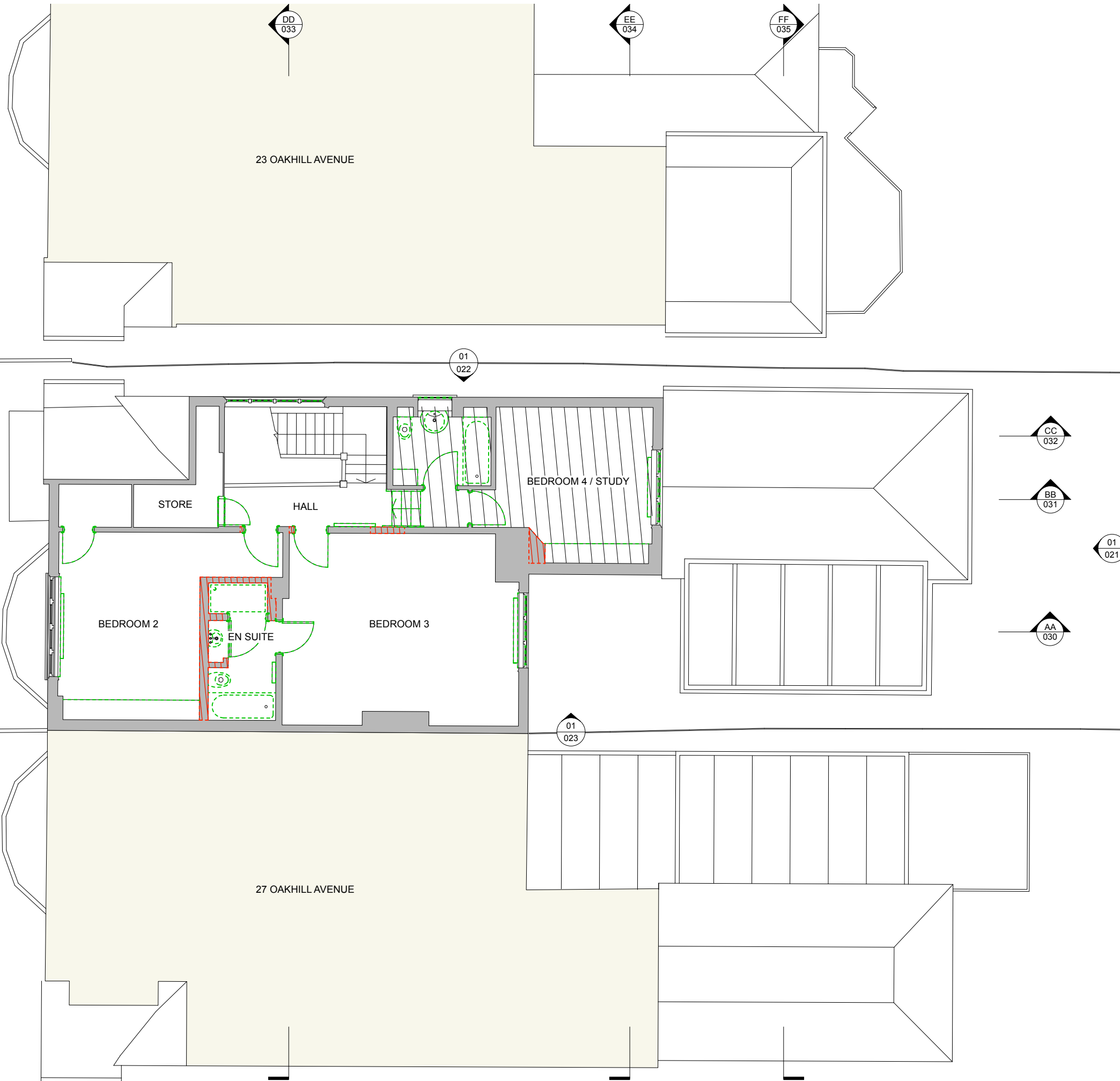
1 EXISTING SECOND FLOOR PLAN 1:100 @ A3
