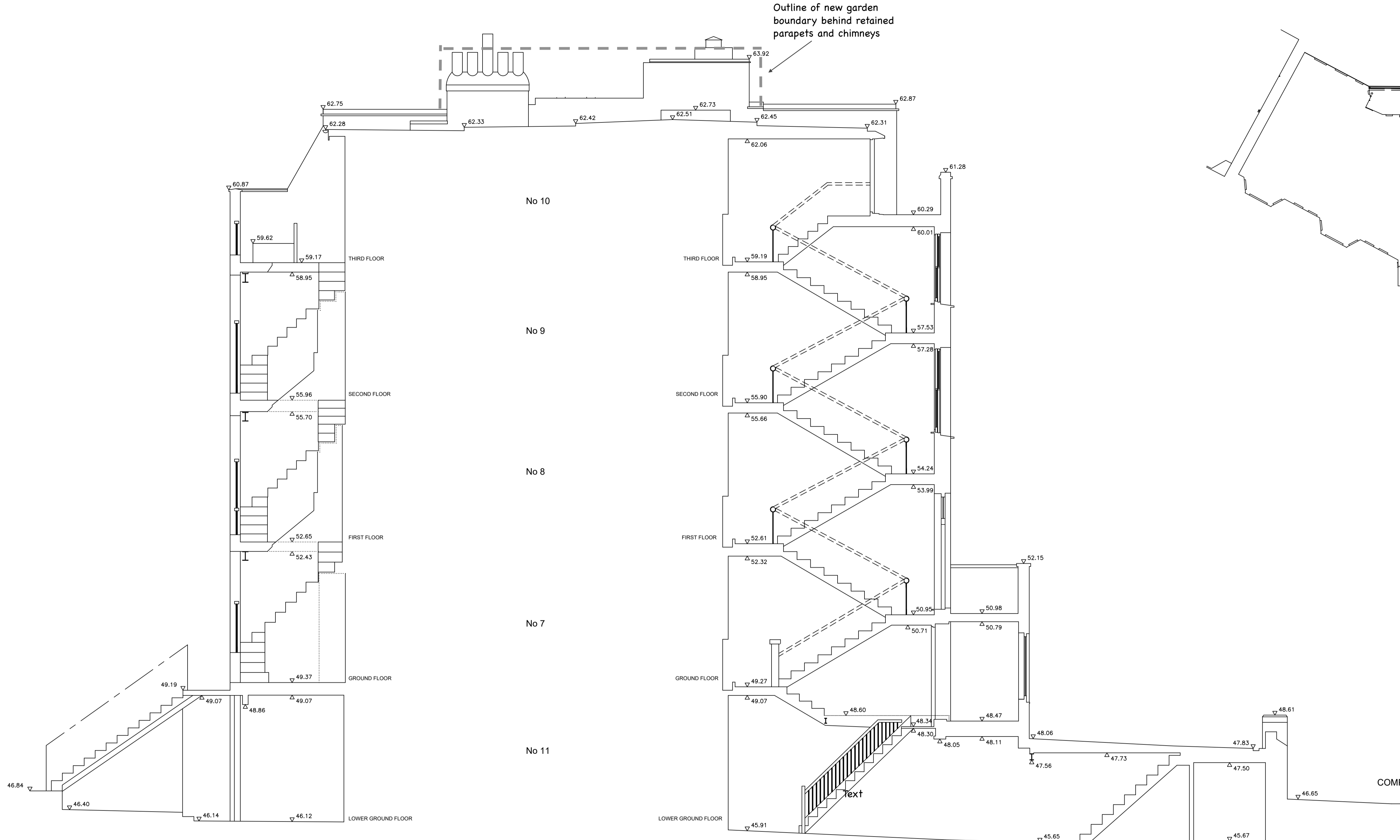
SECTION A-A 45.00m A.O.D.
