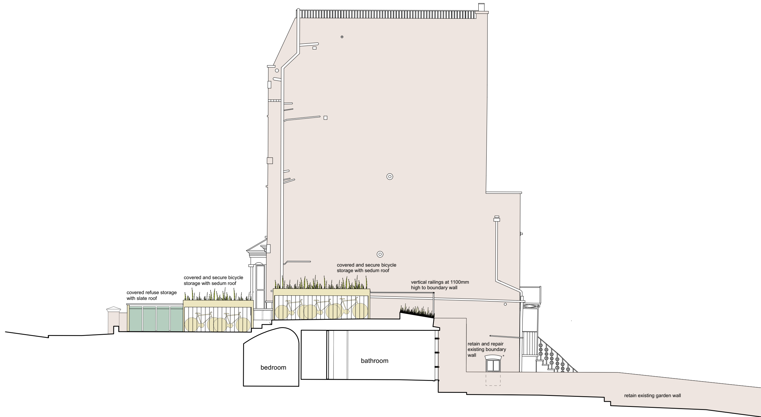
North Elevation of 58 South Hill Park
