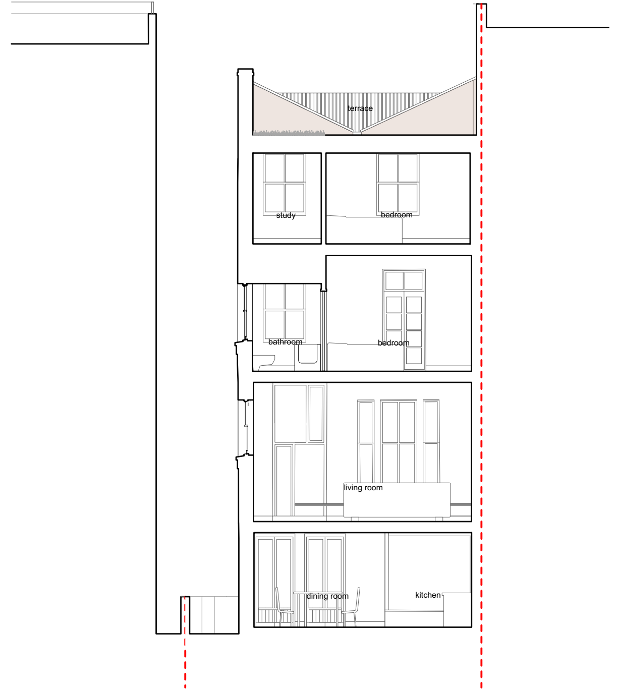
Section BB
