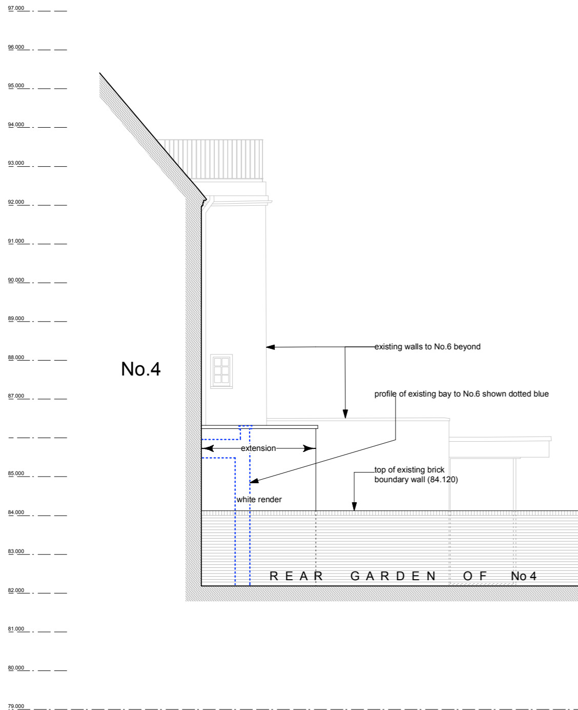
Proposed Side Elevation of Extension as Viewed from No.4
