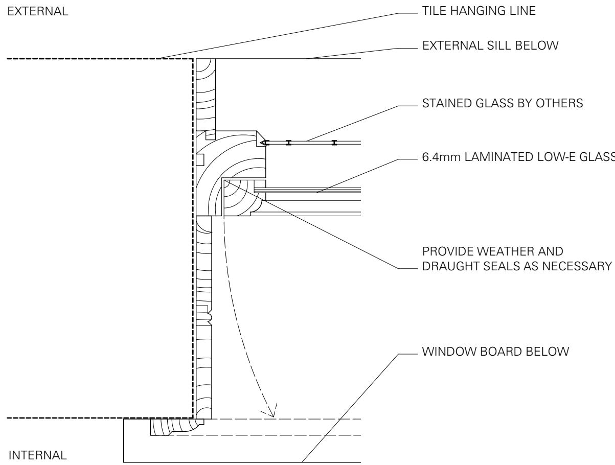
1 TYPICAL JAMB DETAIL. Scale: 1:5
