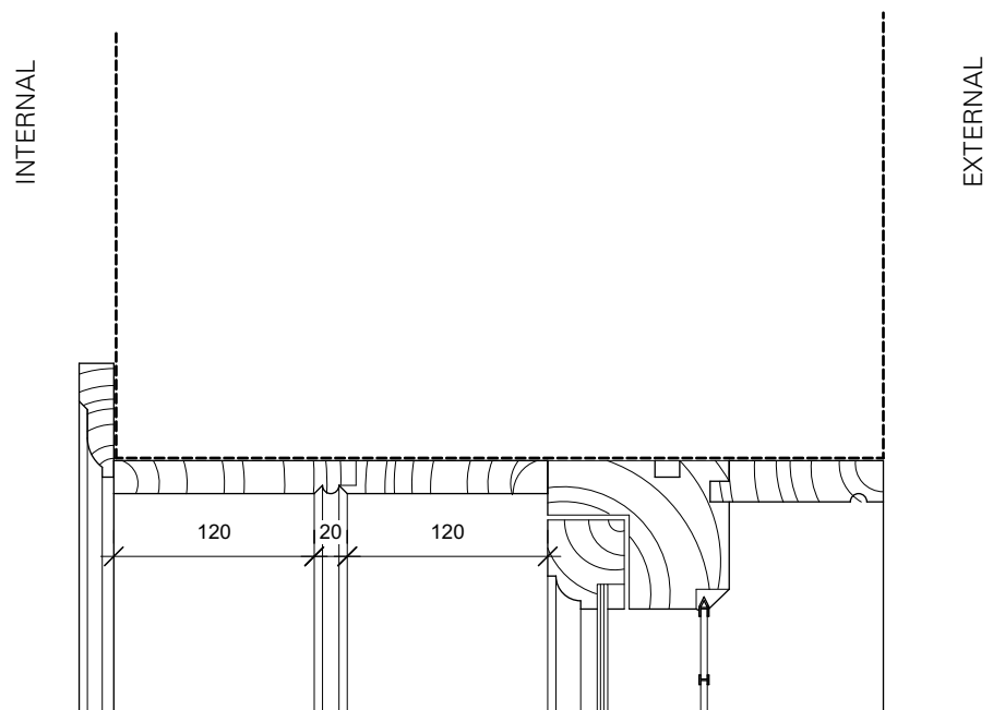
3 TYPICAL HEAD DETAIL. Scale: 1:5
