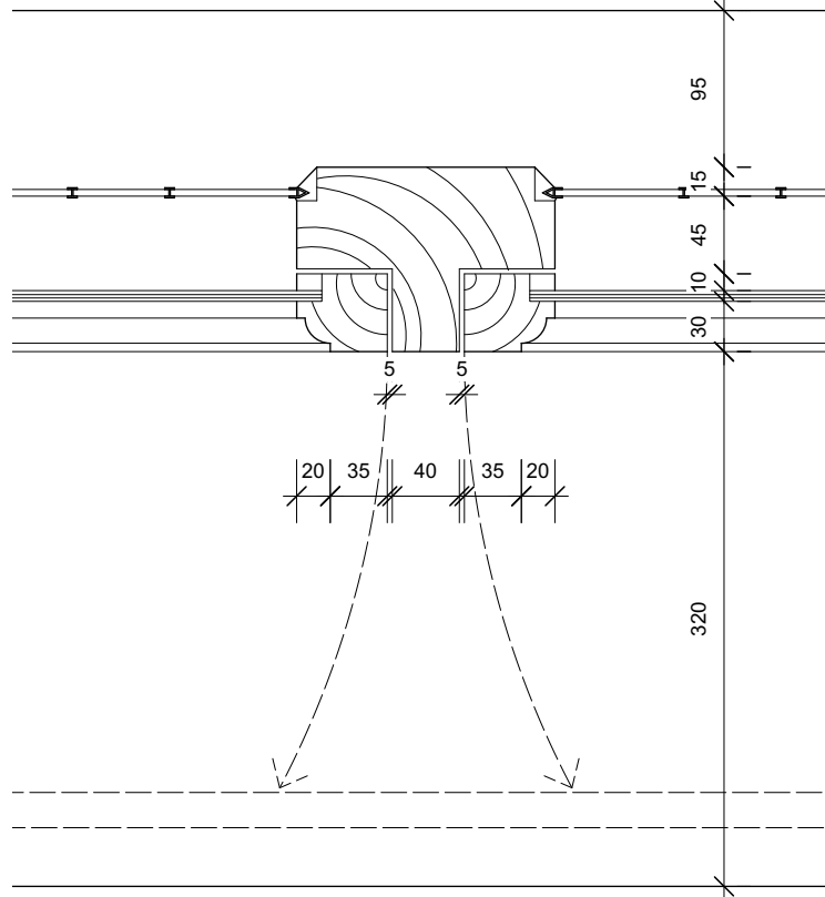
2 MULLION DETAIL (WG.21). Scale: 1:5
