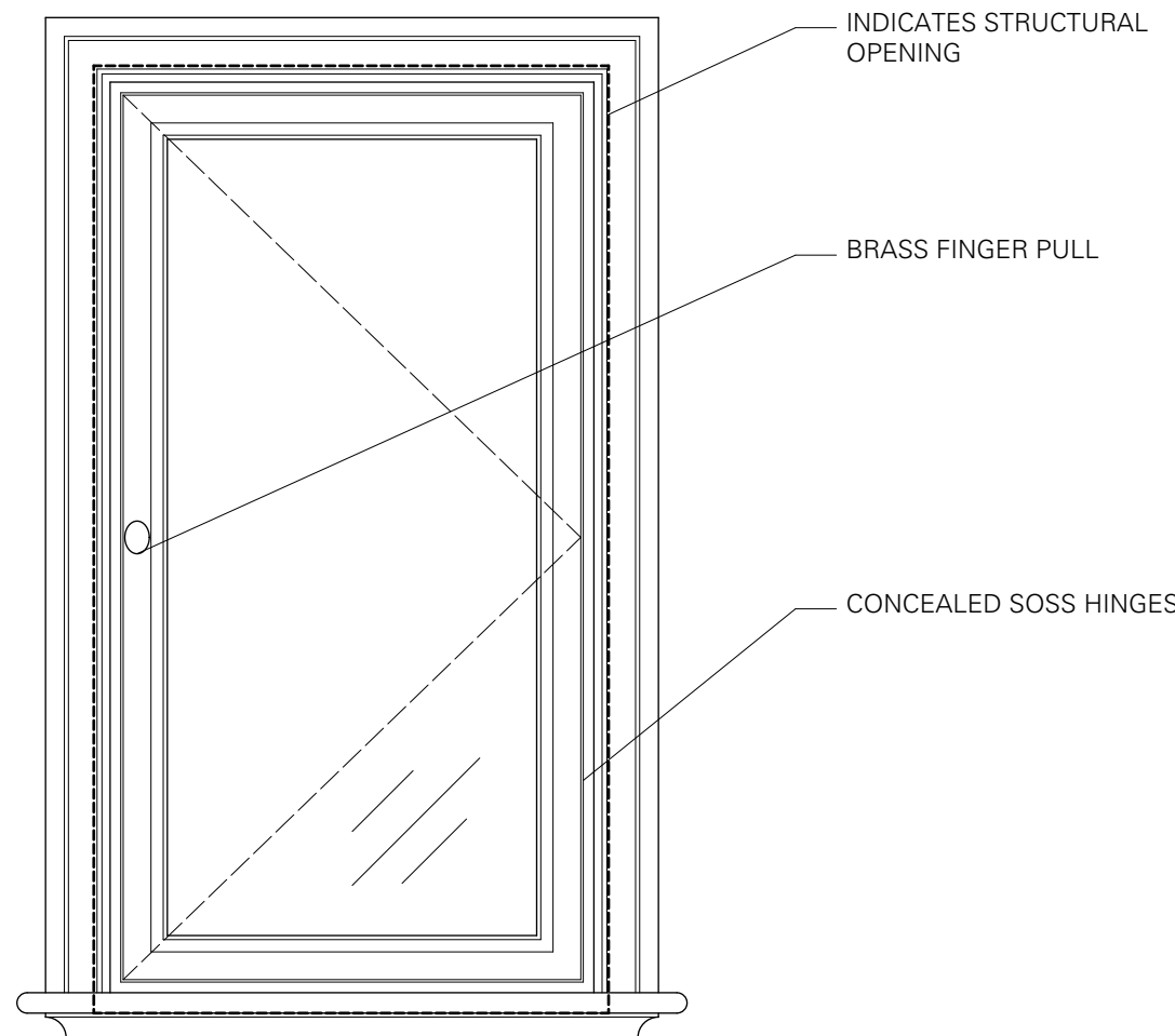
5 INTERNAL ELEVATION - SINGLE CASEMENT Scale: 1:10
