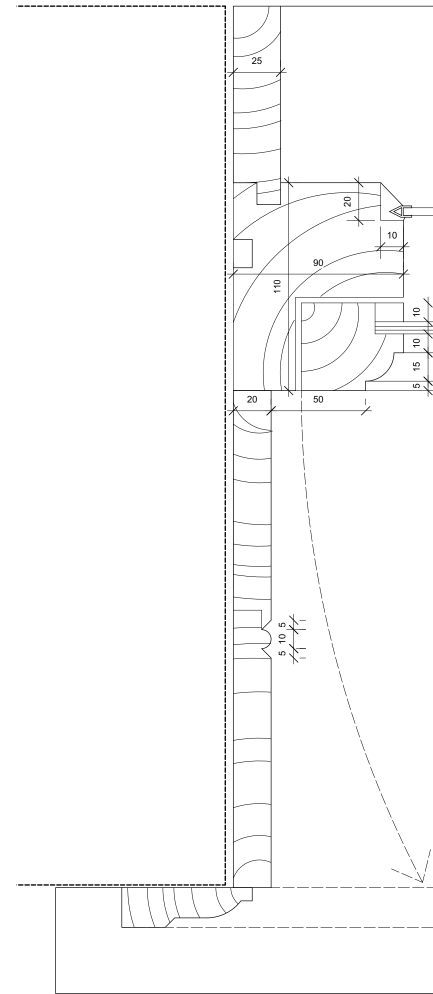
8 TYPICAL JAMB DETAIL. Scale: Half Actual Size
