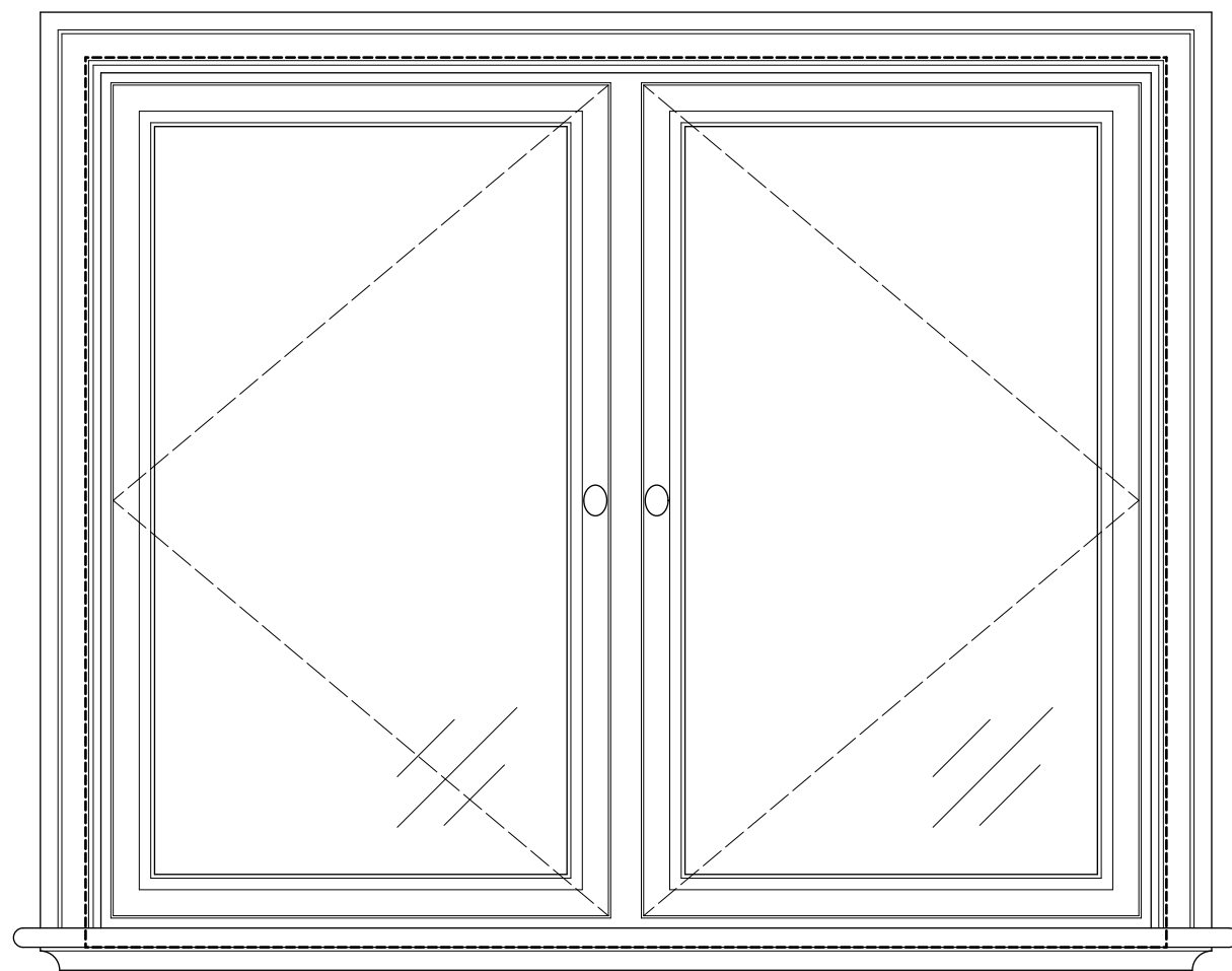
6 INTERNAL ELEVATION - DOUBLE CASEMENT Scale: 1:10
