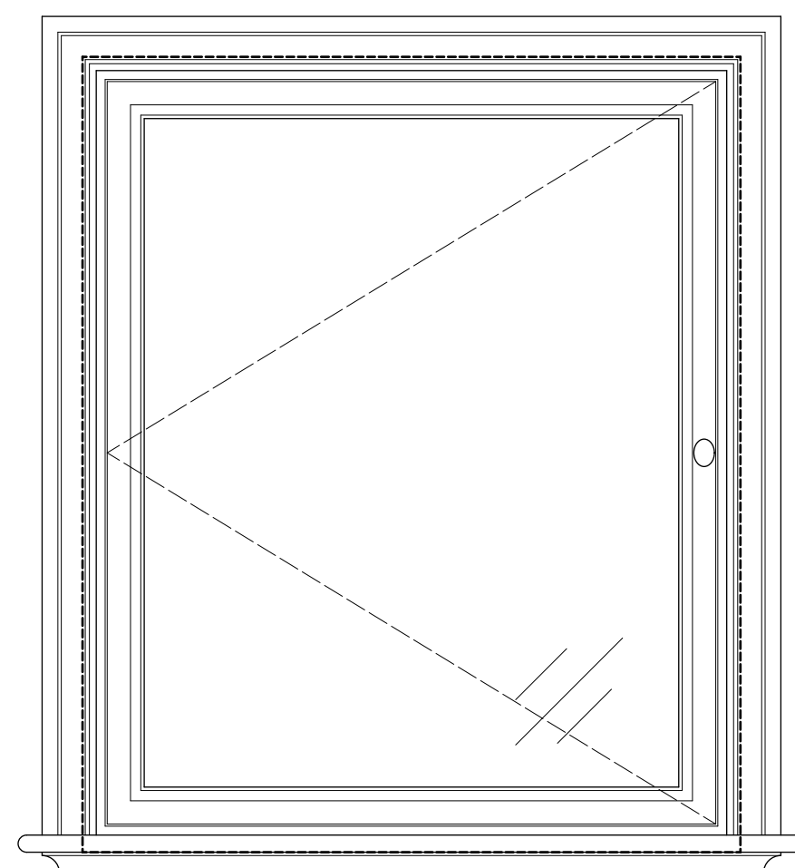
7 INTERNAL ELEVATION - SINGLE CASEMENT Scale: 1:10
