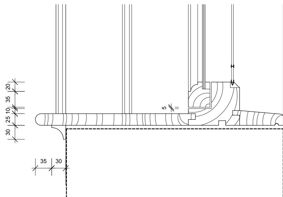
4 TYPICAL SILL DETAIL. Scale: 1:5
