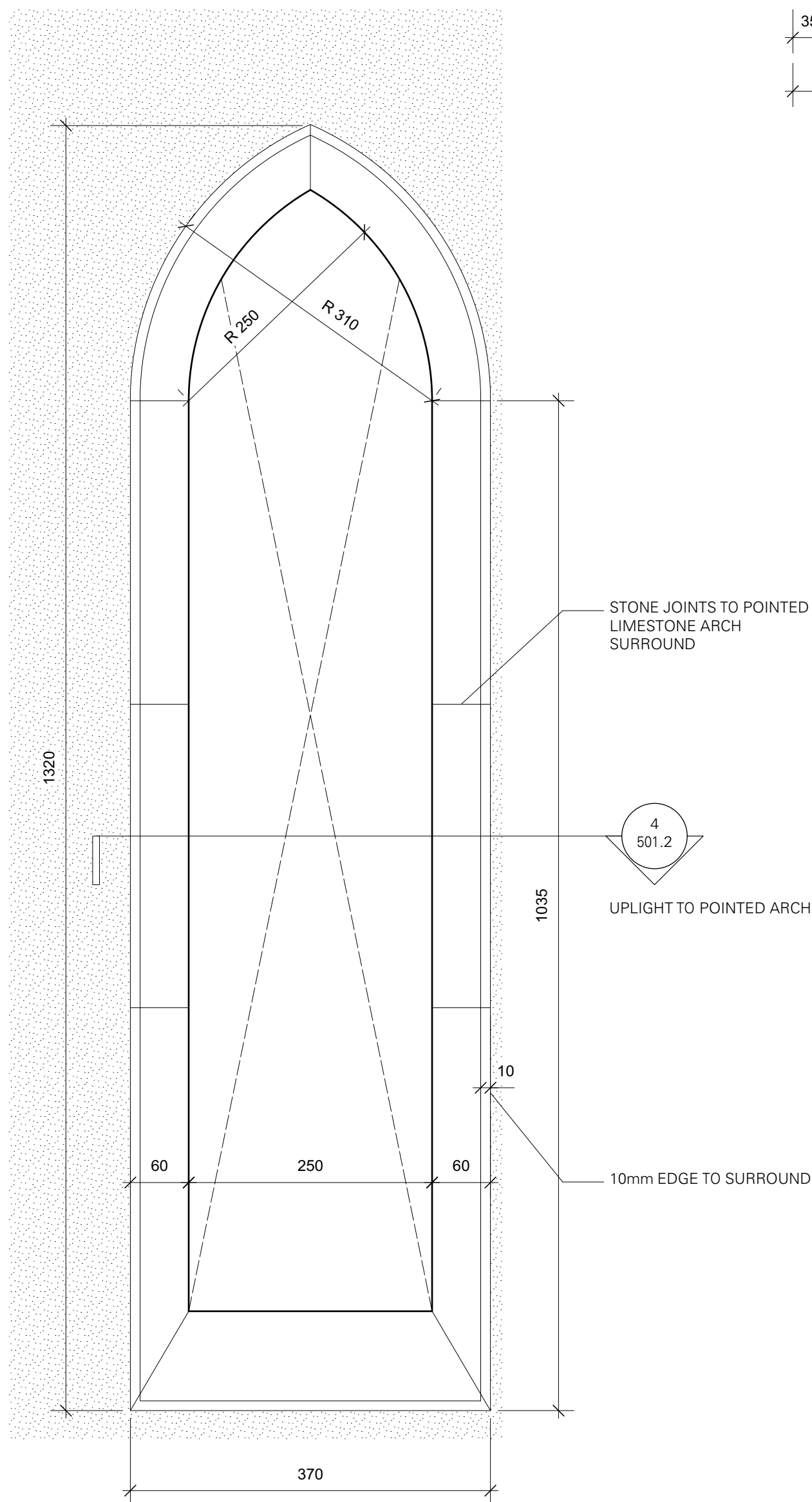
3 POINTED ARCH - SETTING OUT Scale: 1:5
