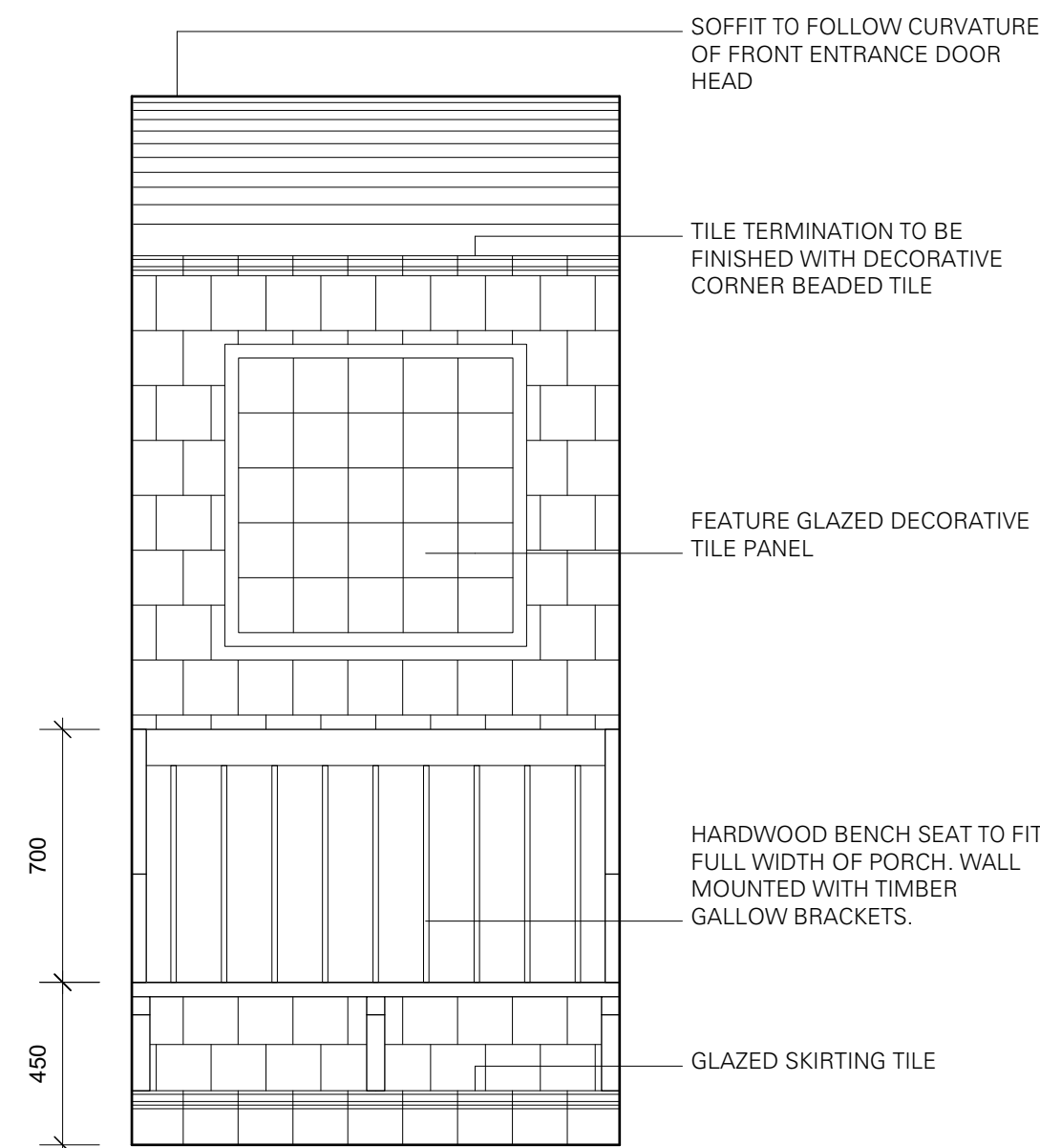
2 ENTRANCE PORCH - INTERNAL ELEVATION Scale: 1:20
