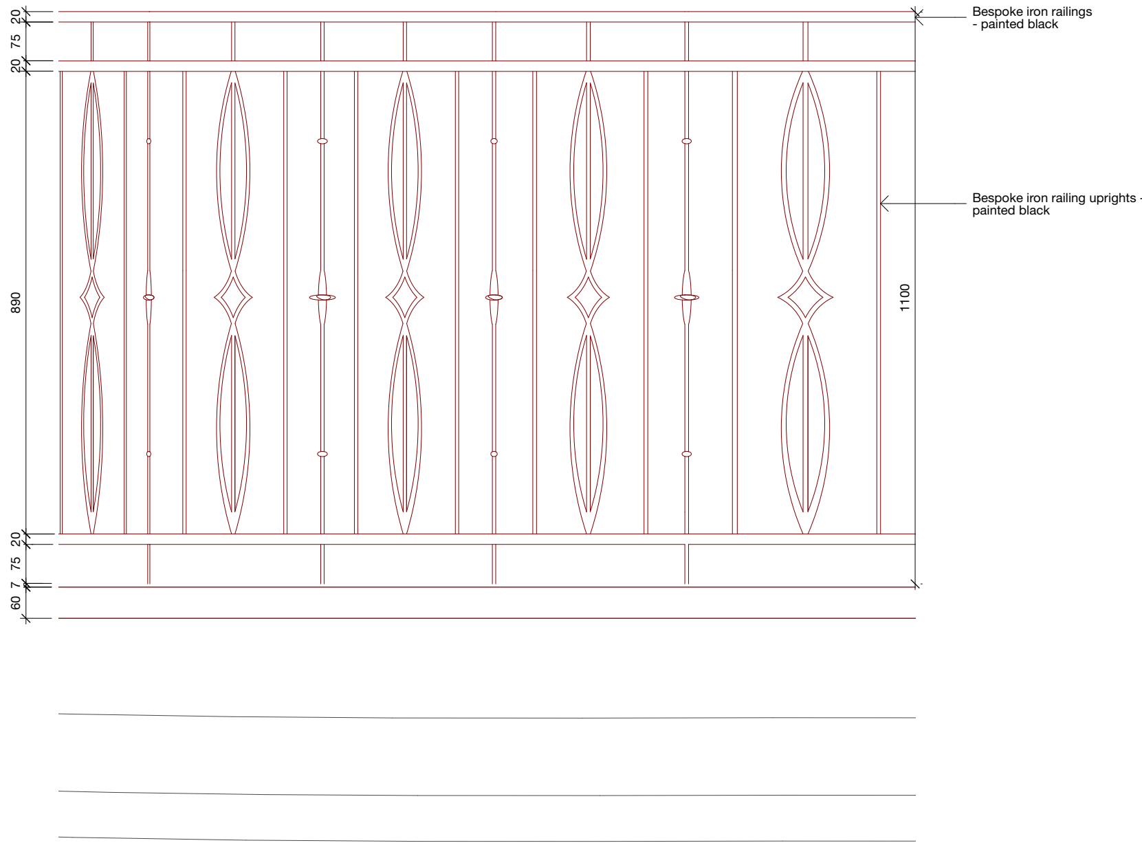
Proposed External Balcony & Stair Railing Elevation PP Scale 1:10
