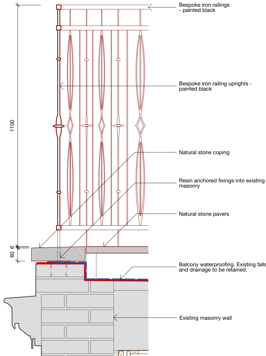
Proposed External Balcony & Stair Railing Section QQ Scale 1:10
