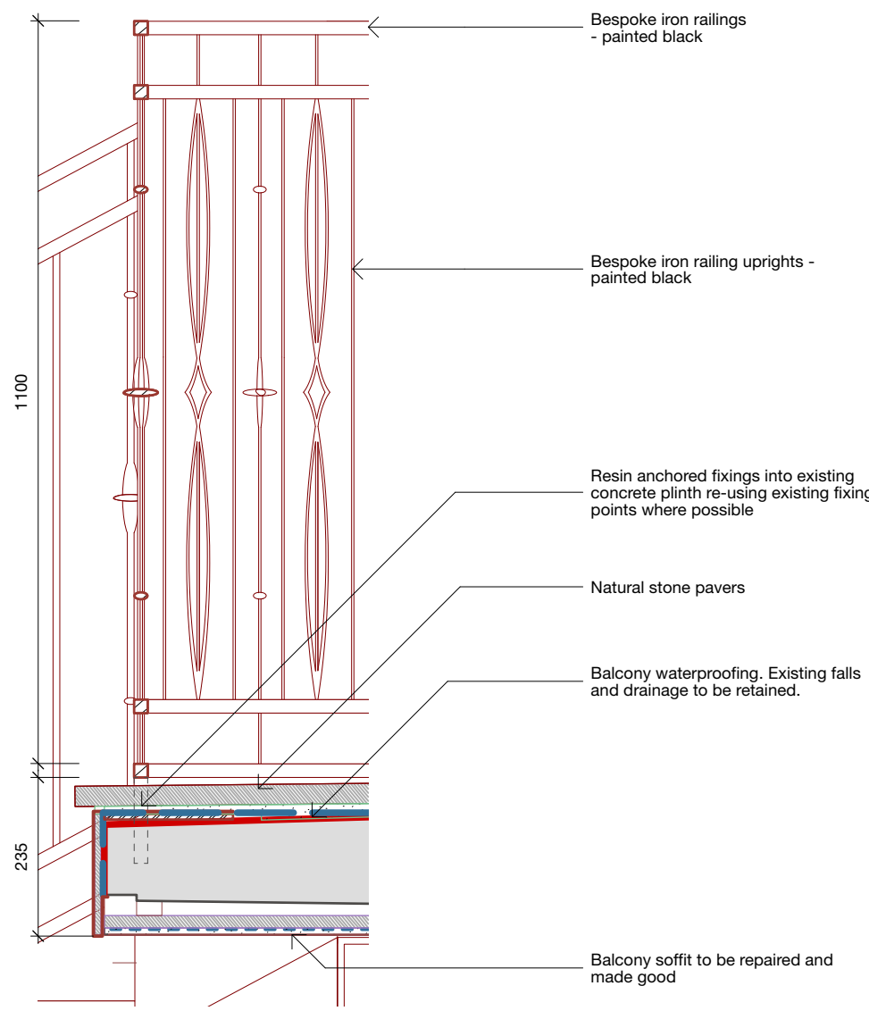
Proposed External Balcony & Stair Railing Section OO Scale 1:10
