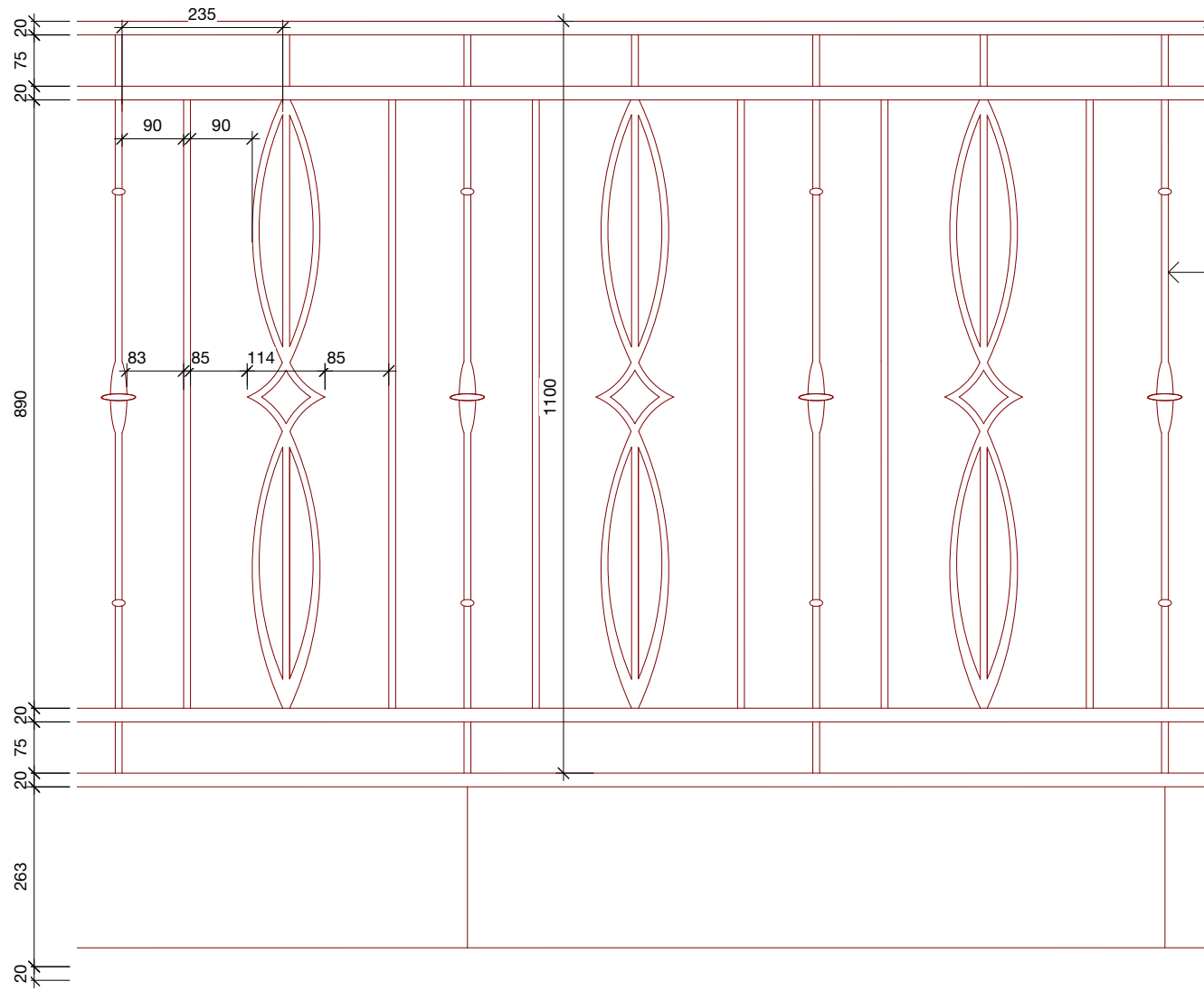
Proposed External Balcony & Stair Railing Elevation NN Scale 1:10
